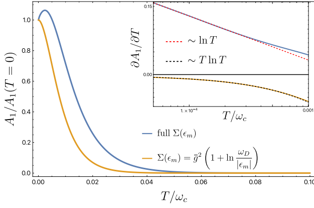
FIG. 2. Numerical evaluation of the first oscillation amplitude A_1(T) and its temperature derivative \partial A_1/\partial T (inset), based on the extended LK formula Eq.(25). For comparison, two different expressions for the fermionic self-energy are used: the full fermion self-energy Eq. (B11), and the marginal Fermi liquid self-energy in the absence of any thermal effects \Sigma(\varepsilon_m) = \bar{g}^2 \varepsilon_m (1 + \ln \omega_D/|\varepsilon_m|) . We note that A_1(T=0) is the same for both cases. The parameters used are \bar{g}^2 = 6 , \Lambda_D = 10\omega_c , v_F/c = 100 .
