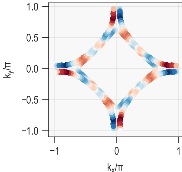
FIG. 5. The calculated RPA superconducting gap structure g_\alpha(\mathbf{k}) for momenta \mathbf{k} on the FS of 326-LNO with g -wave symmetry. The sign of the gap is indicated by the colors (red = positive, blue = negative), and the gap amplitude by its thickness.
