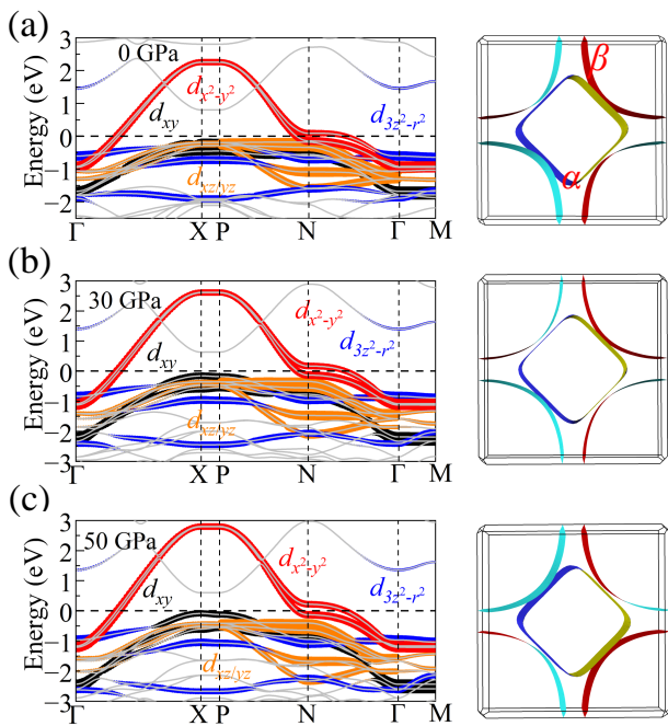
FIG. 7. Projected band structures and FSs of the non-magnetic phase of the I4/mmmm 326-LNO structures without any interaction at (a) 0 GPa, (b) 30 GPa, and (c) 50 GPa, respectively. The weight of each Ni orbital is given by the size of the circles. The Fermi level (zero energy) is marked by the horizontal dashed line. The coordinates of the high-symmetry points of the Brillouin zone are \Gamma = (0, 0, 0) , X = (0, 0, 0.5) , P = (0.25, 0.25, 0.25) , N = (0, 0.5, 0) , and M = (0.5, 0.5, -0.5) .
