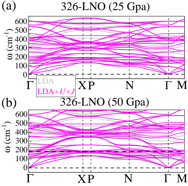
FIG. 8. Phonon spectrum of the I4/mmm phase of 326-LNO at (a) 25 GPa and (b) 50 GPa, respectively. Here, we calculated the phonon spectra for the cases of LDA and LDA plus U and J ( U = 4.75 eV and J = 0.68 eV) with the Liechtenstein formulation within the double-counting item [56], respectively, as distinguished by gray and pink. The coordinates of the high-symmetry points of the Brillouin zone are \Gamma = (0, 0, 0) , X = (0, 0, 0.5) , P = (0.25, 0.25, 0.25) , N = (0, 0.5, 0) , and M = (0.5, 0.5, -0.5) .
