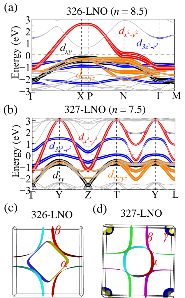
FIG. 2. Projected band structures of the non-magnetic phase of (a) I4/mmmm 326-LNO and (b) Fmmm 327-LNO structures without any electronic interaction, at 25 GPa. The weight of each Ni orbital is given by the size of the circles. The Fermi level (zero energy) is marked by the horizontal dashed line. The coordinates of the high-symmetry points of the Brillouin zone are (a) \Gamma = (0, 0, 0) , X = (0, 0, 0.5) , P = (0.25, 0.25, 0.25) , N = (0, 0.5, 0) , and M = (0.5, 0.5, -0.5) for I4/mmmm 326-LNO and (b) \Gamma = (0, 0, 0) , Y = (0.5, 0, 0.5) , Z = (0.5, 0.5, 0) , T = (0, 0.5, 0.5) , and L = (0.5, 0.5, 0.5) for Fmmm 327-LNO. FSs of the (c) I4/mmmm 326-LNO and (d) Fmmm 327-LNO at 25 GPa. The existence of \gamma pockets is clearly visible in 327-LNO but they are absent in 326-LNO.
