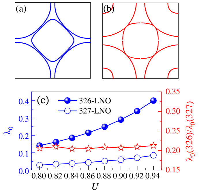
FIG. 4. (a-b) FSs obtained from tight-binding calculations. (a) The hopping and crystal field were obtained from 326-LNO at 25 GPa. Here, the four-band e_g orbital model was considered with the overall filling n = 5 (2.5 electrons per site) in a bilayer lattice. Furthermore, we considered three neighbors of hopping in the xy plane and two neighbors of hopping between layers in our model calculation, while other long-range hoppings are ignored. (b) The hopping and crystal field were obtained for 327-LNO at 25 GPa [9]. (c) The RPA calculated pairing strength \lambda_0 of the leading g -wave pairing state found for 326-LNO and the s_{\pm} -wave state for 327-LNO as a function of U (in units of eV) obtained from the bilayer model. Here we have set U' = U/2 and J = J' = U/4 . The ratio \lambda_0(326\text{-LNO})/\lambda_0(327\text{-LNO}) is also presented in red.
