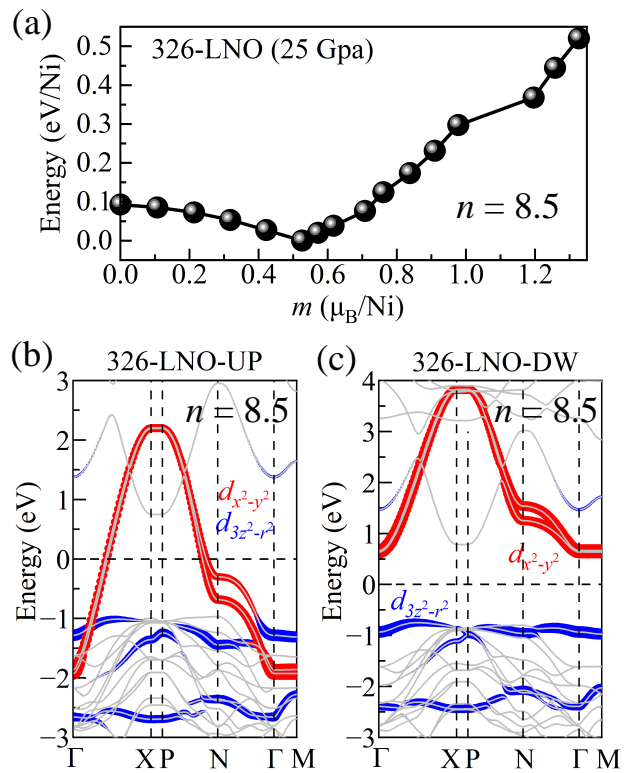
FIG. 3. (a) Total energy as a function of the magnetic moment of the Ni ions for 326-LNO at 25 GPa. (b-c) Projected band structures of the FM phase in the I4/mmmm structural phase of 326-LNO for (b) spin-up and (c) spin-down at 25 GPa. The key e_g orbitals are marked by the red and blue colors. The Fermi level (zero energy) is marked by the horizontal dashed line.
