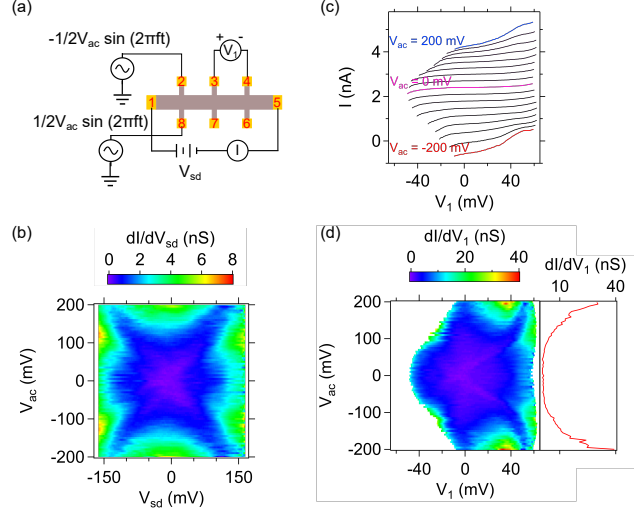
FIG. 4. [nonlocal-Hall] Transport measurements under non-equilibrium excitation. (a) Experimental setup. AC driving with magnitude \frac{1}{2}V_{ac} and frequency f = 1000 Hz are applied differentially to two electrodes labeled 2 and 8 on the left-hand side of the channel device. A quasi-dc voltage V_{sd} is applied between electrodes 1 and 5, swept between -160 mV and 160 mV. (b) Intensity plot of two-terminal conductance versus V_{sd} and V_{ac} . (c) Measured four-terminal conductance in the region between electrodes 3 and 4 for various V_{ac} . Curves are offset for clarity. (d) Four-terminal conductance intensity map versus V_1 and V_{ac} . (e) Linecut of four-terminal conductance at V_{sd} = 0 V.
