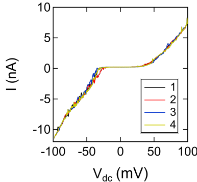
FIG. 2. [fluctuation] Four I - V curves taken consecutively under the same configuration shown in Fig. 1(d). Fluctuations in and around the threshold for conduction are apparent.
