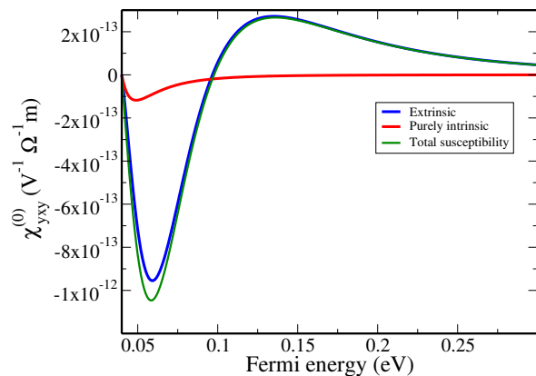
Figure 1: Susceptibility \chi_{yxy}^{(0)} \propto \tau^0 with gap \Delta = 40\text{meV} , tilt t = 0.4 and v_F = 1.6 \times 10^5\text{m/s} . We approximate the Fermi velocity to be the same for all components, v_{0x} = v_{0y} .
