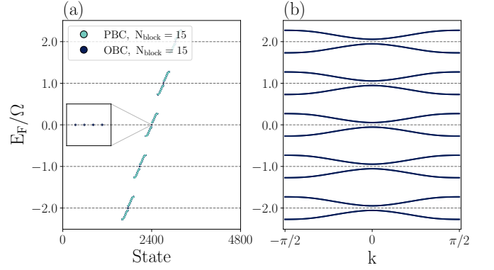
FIG. 1. (a) The quasi-energy spectrum of the direct sum of two identical copies of H(k, t) in Eq. (4). Specifically, we construct the truncated Floquet Hamiltonian \mathcal{H} using the frequency-domain formulation in Eq. (3). Inset: Topological zero edge modes appear within the zero gap, consistent with the expected topological invariant \mathbb{Z} = 2 . (b) The spectrum in periodic boundary conditions. Here, the frequency indices m, n run over a large, but finite range -(N_{\text{block}} - 1)/2 \leq m, n \leq (N_{\text{block}} - 1)/2 , where N_{\text{block}} is much larger than the frequency space localization of the Floquet states. The parameters used are T = 1 , J_1 = \Omega = 2\pi , J_2/J_1 = 0.9 , J_3/J_1 = J_4/J_1 = 0.1 , and N_{\text{block}} = 15 .
