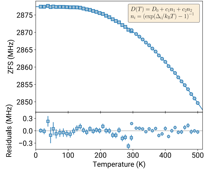
FIG. 2. Zero-field splitting as a function of temperature. Top: Data points show the average zero-field ODMR center frequency of several individual NV centers at each temperature. Square (circle) data points indicate measurements conducted in low(high)-temperature operation mode using the same 5 NV centers belonging to set A (B). The two sets are mutually exclusive. Standard error bars are smaller than the data points. Solid line shows fit of the proposed model (Eq. (3), reproduced in top right corner) to the experimental data, with fit parameters presented in Table I. Bottom: Residuals.
