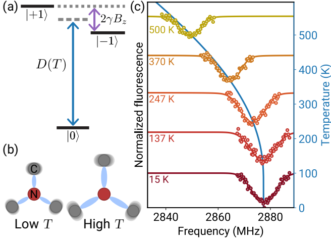
FIG. 1. Temperature-dependent energy levels of the nitrogen-vacancy (NV) center. (a) Electronic ground-state level structure of the negatively charged NV center. In the absence of external fields, the |m_s = \pm 1\rangle spin sub-levels are degenerate with energy D(T) above |m_s = 0\rangle , where D(T) is the temperature-dependent zero-field splitting (ZFS). The |\pm 1\rangle levels are commonly split by a magnetic field B_z applied along the NV axis. (b) Illustration of the origin of the ZFS temperature dependence. In this 2D diagram, the NV center is projected onto the plane perpendicular to the NV axis, showing only the nitrogen (red) and carbon atoms (gray) nearest the vacancy. The cartoon is not to scale, with the effect of temperature highly exaggerated and only a single vibrational mode depicted for clarity. The ground-state electronic spin density is localized to dangling bonds (blue) between the carbon atoms and the vacancy [19]. Thermal expansion and increases in vibrational amplitudes both reduce the spin-spin interaction that leads to the ZFS [19]. We find that each of these effects can be described by a weighted sum of phonon occupation numbers. (c) Temperature dependence of optically-detected magnetic resonance. Data points show fluorescence from a single NV center under zero applied field after optical spin polarization and a microwave pulse at the frequency indicated by the x -axis. Solid lines are fits to double-Voigt profiles [20]. Each data set is offset such that the minimum of the fit aligns with the appropriate temperature on the righthand y -axis. The blue line shows the ZFS as a function of temperature according to a fit of the proposed model, Eq. (3), to the full set of experimental data.
