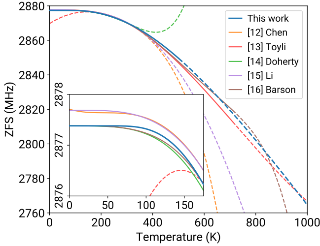
FIG. 4. Comparison to prior models of the ZFS temperature dependence. Prior models are reproduced from Refs. [12–16] according to the fit parameters published in those works. The line for each model turns from solid to dashed outside the temperature range covered by the experimental data on which the model was fit. See Sec. IV of the Supplemental Material for details regarding prior results [20]. Inset: Low-temperature behavior of models.
