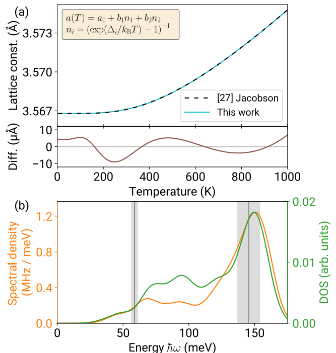
FIG. 3. Physical motivation for proposed model of the zero-field splitting temperature dependence. (a) Diamond lattice constant as a function of temperature. Dashed black line indicates the diamond lattice constant calculated from the results of Ref. [27]. Fitting Eq. (11) (reproduced in upper left corner) to this curve yields an excellent approximation of the lattice constant with just three free parameters (cyan line). The form of Eq. (11) matches that of Eq. (3). Bottom: Residuals. (b) Second-order spin-phonon spectral density (orange) and phonon density of states (DOS, green) calculated from the results of Ref. [21]. The spectral density describes the shift of the ZFS induced by the second-order effects of phonons at a given energy. The spectral density closely matches the DOS, suggesting that both first- and second-order contributions to ZFS shifts can be modeled by a weighted sum of occupation numbers of phonon modes with representative energies. The energies extracted from the fit of Eq. (3) to the experimental ZFS data (gray lines and \pm 1\sigma intervals) roughly match the locations of prominent features in the spectral density and DOS. Note that the spectral density is negative everywhere. The plot shows its magnitude.
