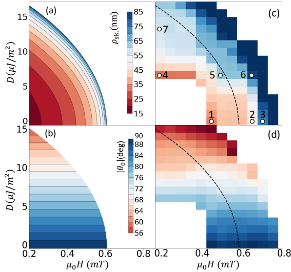
FIG. 4. The skyrmion characteristics in the low DMI regime for d = 5 nm, A = 20 pJ/m, M_s = 10^5 A/m, and K_u = 6346 J/m 3 corresponding to Q = 1.01 : (a) Skyrmion radius r_{\text{sk}} and (b) skyrmion rotation angle |\theta_0| from (6) and (5); (c) skyrmion radius and (d) skyrmion rotation angle from MuMax3 simulations on a 2048 \times 2048 nm 2 square box with mesh size 2 \times 2 \times 5 nm. The dashed line is the line of zero bursting barrier defined in (10).
