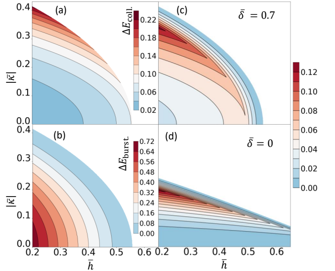
FIG. 3. Skyrmion collapse \Delta E_{\text{coll}} (a) and bursting \Delta E_{\text{burst}} (b) energy barriers (in units of Ad ) for the intermediate thickness regime with \bar{\delta} = 0.7 . Also shown is the effective barrier \Delta E = \min(\Delta E_{\text{coll}}, \Delta E_{\text{burst}}) , which illustrates the optimal stability region against collapse and bursting for \bar{\delta} = 0.7 (c) and for the ultrathin film with \bar{\delta} = 0 (d).
