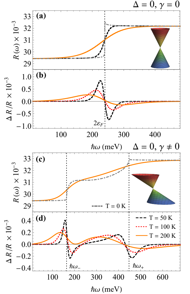
FIG. 2. Optical reflectivity R(\omega) and its thermal derivative \Delta R/R for several temperatures of the sample at normal incidence, corresponding to (a)-(b) graphene and (c)-(d) a gapless tilted anisotropic system (borophene 8- Pmmn ). The insets illustrate the energy bands in each case. We use \varepsilon_F = 120 meV and \Delta T = 1 K.
