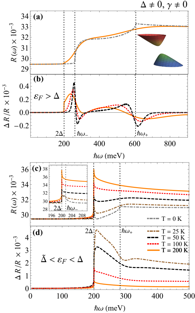
FIG. 4. Optical reflectivity and thermal derivative of a massive tilted Dirac system ( \Delta = 100 meV) for several temperatures when the Fermi energy lies (a)-(b) above the gap \varepsilon_F > \Delta (with \varepsilon_F = 170 meV) and (c)-(d) in the indirect zone \tilde{\Delta} < \varepsilon_F < \Delta (with \varepsilon_F = 95 meV). The velocities v_i are taken as in borophene, and \Delta T = 1 K.
