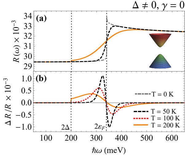
FIG. 3. (a) Optical reflectivity R(\omega) and (b) its thermal derivative \Delta R/R for several temperatures of the sample, corresponding to gapped graphene, with \varepsilon_F > \Delta . We take \varepsilon_F = 170 meV, \Delta = 100 meV, and \Delta T = 1 K.
