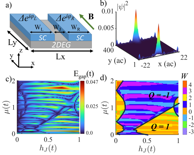
Figure 1. a) Schematic diagram of the planar Josephson junction heterostructure. The 2DEG is covered by d -wave superconductors, except for a junction of width W_J between the two superconductors. In b) the probability function ( |\psi|^2 ) of MBS at \mu = 1.32t and h_J = 0.6t is plotted. c) The energy gap as a function of the Zeeman field h_J in the junction and \mu . d) The topological invariants Q ( \mathbb{Z}_2 ) and W ( \mathbb{Z} ) as a function of the Zeeman field h_J in the junction and \mu . The colors show the value of the W invariant. The black lines separate the regions with Q = -1 and 1 . The W invariant only changes between odd (even) values for Q = -1 (1) regions. We used the parameters: L_y = 400a_c , W_J = 5a_c , W_L = W_R = 20a_c , \Delta_0 = 0.3t , \Delta'_0 = 0.0 , h_{SC} = 0 , and the phase difference \Delta\phi = \pi .
