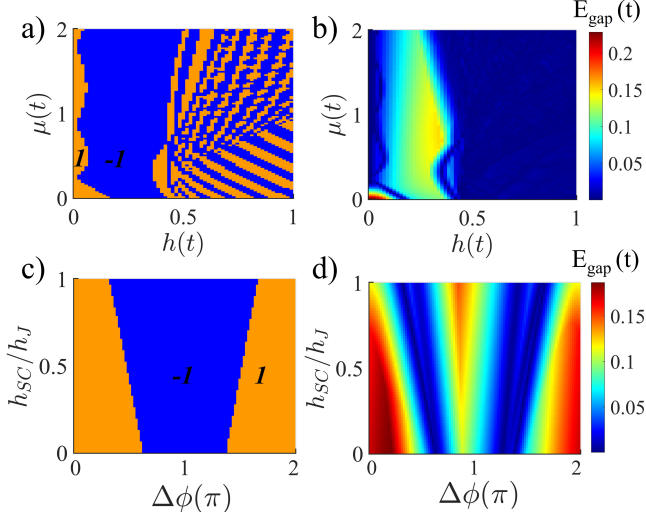
Figure 3. The Zeeman field is applied to the whole system. a) The Q topological invariant as a function of h and \mu where h_J = h_{SC} = h for the phase difference \Delta\phi = \pi . The blue color shows the topological region ( Q = -1 ). b) The energy gap E_{gap} as a function of h and \mu where h_J = h_{SC} = h for the phase difference \Delta\phi = \pi . c), d) The Q topological number and the energy gap as a function of the ratio h_{SC}/h_J and \phi for \mu = 1t . We used the parameters: \Delta_0 = 0.3t , \Delta'_0 = 0.0 , \beta = \pi/4 , h_J = 0.2t , W_J = 5a_c , and W_L = W_R = 40a_c .
