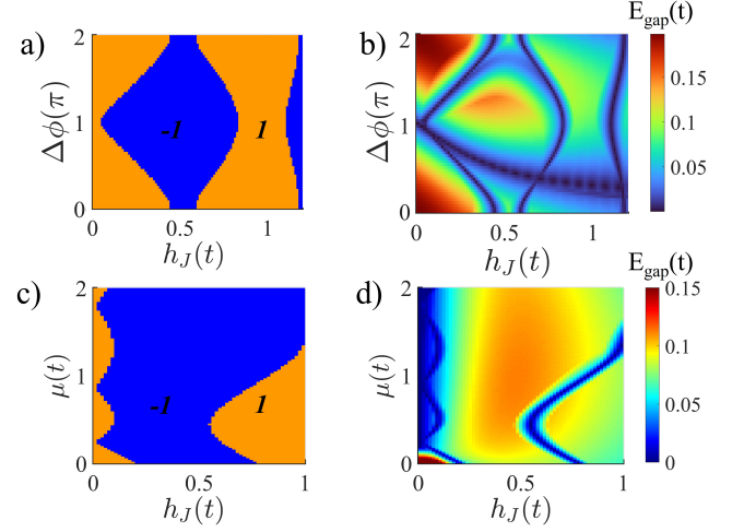
Figure 2. Phase diagrams for d + is pairing ( \beta = \pi/4 ). a) The Q topological number ( \mathbb{Z}_2 ) as a function of h_J and \Delta\phi for \mu = 1t . b) The energy gap E_{\text{gap}} as a function of h_J and \Delta\phi for \mu = 1t . (The dark blue line extending from left to right has a small gap, which is why no corresponding topological phase change exist in a)) c) Phase diagram of the Q topological number as a function of h_J and \mu for the phase difference \Delta\phi = \pi . d) The energy gap E_{\text{gap}} as a function of h_J and \mu for the phase difference \Delta\phi = \pi . We used the parameters: h_{SC} = 0 , \Delta_0 = 0.3t , \Delta'_0 = 0.0 , W_J = 5a_c , W_L = W_R = 40a_c .
