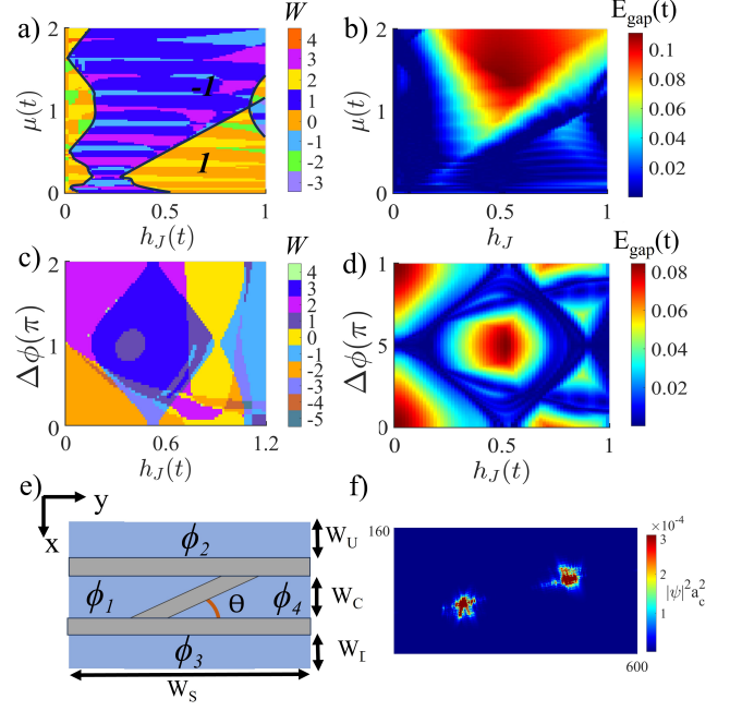
Figure 4. a) The topological invariant W as a function of h_J and \mu for \Delta\phi = \pi . The black line shows the outlines of Q = -1 and Q = 1 regions. b) The gap E_{gap} of a JJ with periodic boundaries as a function of h_J and \mu for \Delta\phi = \pi . c) The topological number W as a function of h_J and \Delta\phi for \mu = 1t . d) The gap E_{gap} of a JJ with periodic boundaries as a function of h_J and \Delta\phi for \mu = 1t . We used the parameters: W_J = 5a_c , W_L = W_R = 20a_c . e) and f) Modified JJ structure and |\psi|^2 of the lowest eigenvalue corresponding to MBS. The phases of four superconducting regions are set to: \phi_1 = \phi_2 = \pi/2 , \phi_3 = \phi_4 = -\pi/2 . Dimensions used: W_U = W_D = W_C = 50a_c , W_S = 600a_c , W_J = 5a_c . Other parameters used: h_J = 0.4t , h_{SC} = 0 , \mu = 2t , \Delta_0 = 0.3t , \Delta'_0 = 0.06t , \theta = \arctan(1/9) \approx \pi/9 .
