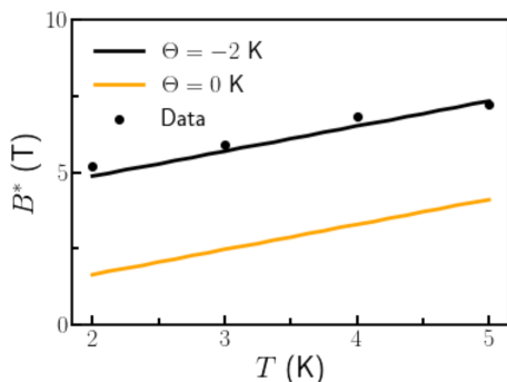
FIG. 5. The magnetic field where the SSE is maximized is plotted ( T = 2, 3, 4 \text{ K} from Ref. [14] and T = 5 \text{ K} from Ref. [13]) which depends only on the spin Seebeck coefficient. The theory contains a single, constant undetermined parameter: the Curie-Weiss temperature \Theta_{CW} , after we took S = 7/2 for GGG.
