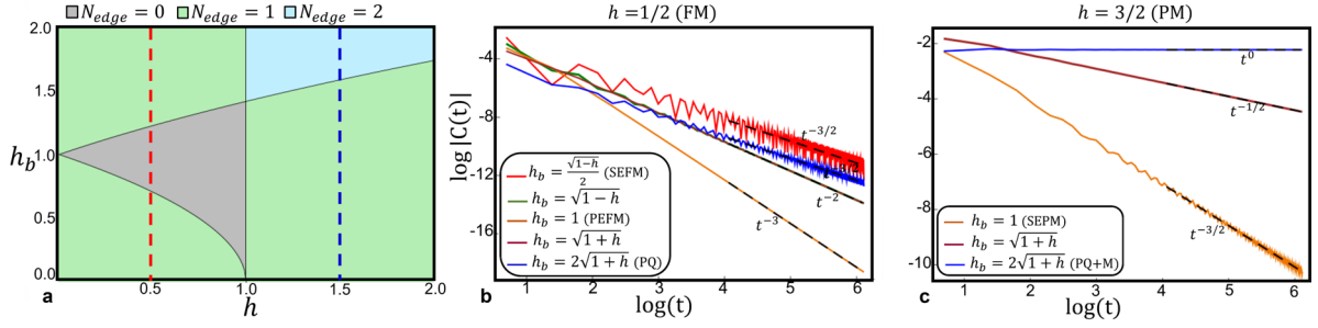
FIG. 2: (a) Phase diagram representing the edge states in the presence of boundary field h_b . (b,c) Plots of autocorrelation function for h = 0.5 and h = 1.5 with different values of h_b taken across the different phases of edge states represented by red and blue lines in the phase diagram, respectively. Power laws are shown as guides to the eye and match those shown in Fig. 1.
