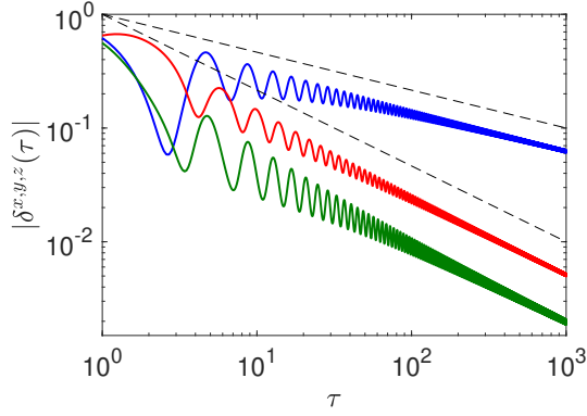
FIG. 1. Numerical data for deviations from the adiabatic value for spin components x , y and z (blue, red and green) from top to bottom after quenching to the critical point ( g = 1 ) from the FM ( g_0 = 0 ) phase. The black dashed lines depict the \tau^{-1/3} and \tau^{-2/3} scalings.
