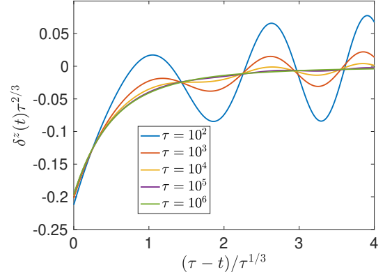
FIG. 2. Temporal data collapse of \delta^z(t) close to the CP for various ramp rates after a ramp from the FM ( g_0 = 0 ). The data is obtained from the numerical solution of Eq. (4) Deviations from zero start to appear at times \sim \tau^{1/3} before reaching the CP. Similar data collapse characterizes the other spin components.
