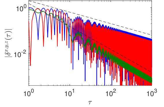
FIG. 3. Numerical solution of the deviations from the adiabatic value for spin components x , y and z (blue, red and green) from top to bottom after quenching from FM ( g_0 = 0 ) to PM ( g = 3 ). The black dashed lines depict the \tau^{-1/2} and \tau^{-1} scalings obtained analytically.
