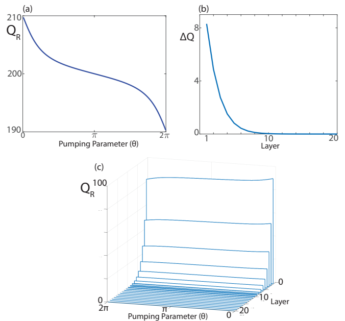
FIG. 3. (a) Total charge on the right half of the system (positive x -direction) as a function of charge pumping parameter \theta (i.e., the flux threaded in the y -direction) for twenty Chern insulator layers. (b) Amount of charge pumped on each layer after one cycle. (c) Total charge on the right half of the system resolved vs. layer. Note that the total charge is exponentially localized on one surface, and the variation of charge as a function of \theta is strongest on that surface and decays away.
