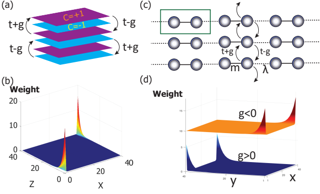
FIG. 4. (a) Schematic illustration of a \mathbb{Z}_2 bi-directional skin effect model built from bi-layers with opposite Chern-number (b) the probability density of the negative energy boundary states at a fixed value of k_y for OBC in x, z and PBC in y . The subspace of boundary states at -k_y would have the corners flipped. (c) Schematic illustration of 2D model built from Su-Schrieffer-Heeger chains parallel to \hat{x} stacked with HN coupling along \hat{y} . (d) Probability density for negative energy boundary modes for OBC in x, y when g < 0 and g > 0 . The plot for g < 0 has been manually shifted upward by a weight of 10 for easier visibility.
