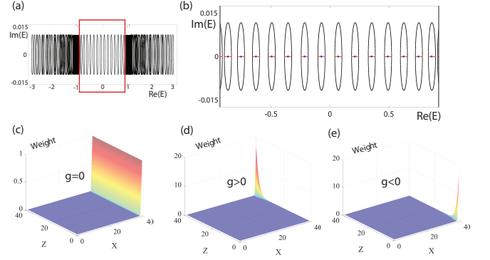
FIG. 2. (a) Complex energy spectrum with PBC in z , and OBC in x, y . (b) Zoom in on the boundary state region from (a) in red box. Blue stars have t = g = 0 , red lines have t \neq 0, g = 0 , and black lines have t, g \neq 0 . (c, d, e) sum of probability densities of the negative \text{Re}(E) boundary states for (c) g = 0 , (d) g > 0 , and (e) g < 0 .
