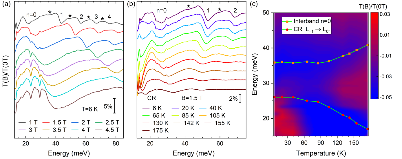
FIG. 2. (a) Magnetic field dependence of normalized magneto-transmission spectra, T(B)/T(0T) , of ZrTe 5 measured at 6 K from 1 T to 4.5 T. (b) Temperature-dependent magneto-transmission spectra, T(B)/T(0T) , of ZrTe 5 from 6 K to 175 K at 1.5 T. The integer index n labels the interband LL transitions L_{-n(-n-1)} \rightarrow L_{n+1(n)} . The asterisk symbol (*) indicates the second set of LL transitions, a hallmark of the STI phase in ZrTe 5 at low temperatures [36]. A CR mode emerges at elevated temperatures, which can be attributed to the L_{-1} \rightarrow L_0 transition. (c) False color map of the temperature evolution of the normalized magneto-transmission spectra, T(B)/T(0T) , of ZrTe 5 measured at 3 T. The symbols and lines denote the CR (red symbol) and interband n = 0 (orange symbol) transition energies calculated from the band parameters extracted from the model fitting of the interband LL transitions. The corresponding raw spectra of (c) are shown in Figure 6 in Appendix. All measurements are performed with B \parallel b -axis. The spectra are offset vertically for clarity in (a) and (b).
