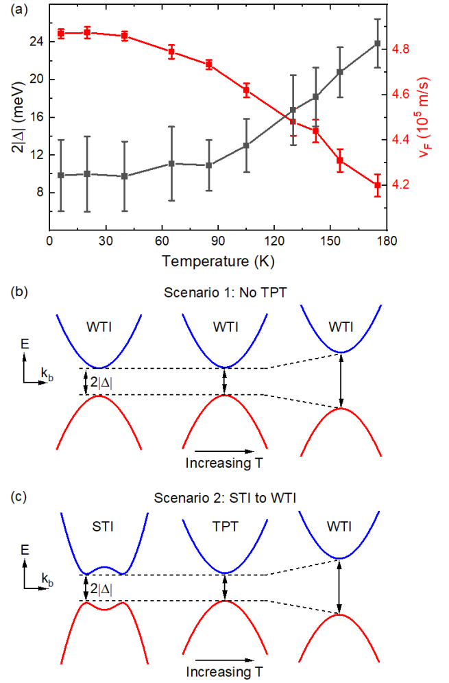
FIG. 4. (a) Temperature dependence of the extracted Fermi velocities and band gaps. The error bars are determined from the LL transition energy uncertainties. (b,c) Schematic drawings of the band structure evolution as a function of temperature for two possible scenarios that can describe our experiment.
