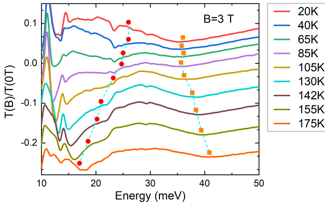
FIG. 6. Temperature-dependent normalized magneto-transmission spectra measured from 20 K to 175 K at 3 T. The spectra are offset vertically for clarity.
