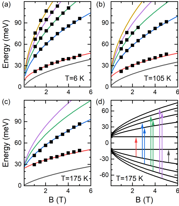
FIG. 3. Magnetic field dependence of LL transitions at selected temperatures of (a) T = 6 K, (b) 105 K, and (c) 175 K. The black squares are the experimentally extracted transition energies, and the size of the squares is larger than the uncertainty of the transition energies. The solid lines are the best fits to the data using the massive Dirac fermion model (1). (d) Representative Landau fan diagram for T = 175 K. The LLs are labeled by the index n = 0, 1, 2, \dots , and their corresponding LL transitions L_{-n(-n-1)} \rightarrow L_{n+1(n)} are color-coded consistent with those in (a)-(c). Due to the electron-hole symmetry at low fields, the \Delta n = \pm 1 transitions degenerate.
