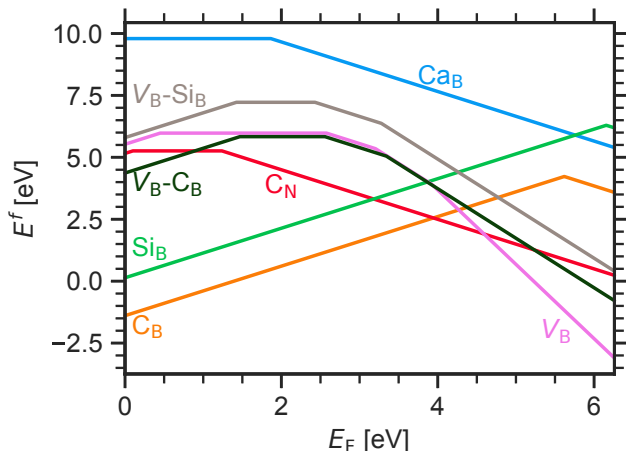
FIG. 1. Formation energies E^f of the substitutional impurities ( C_B , C_N , Si_B , and Ca_B ), V_B , and impurity-vacancy complexes ( V_B - C_B and V_B - Si_B ) as a function of the Fermi level E_F .
