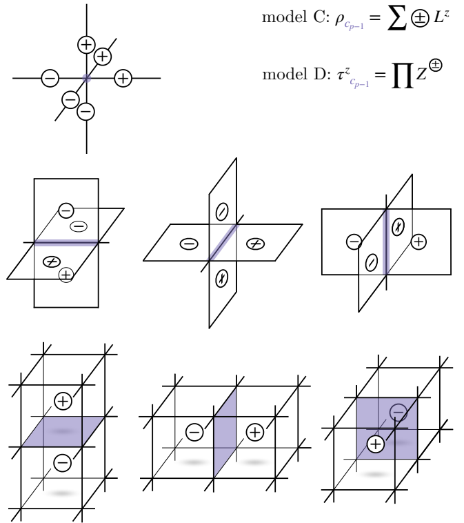
FIG. 6. Graphical representation of \rho_{c_{p-1}} in model C (42) and \tau_{c_{p-1}}^z in model D (26) in 3d space for (1st row) p = 1 , (2nd row) p = 2 , and (3rd row) p = 3 . The (p-1) -cell c_{p-1} is colored purple. The \pm disks on the p -cells denote the sign in front of L_{c_p}^z in the sum for \rho_{c_{p-1}} , or whether Z_{c_p} is Z^+ \equiv Z or Z^- \equiv Z^\dagger in the product for \tau_{c_{p-1}}^z .
