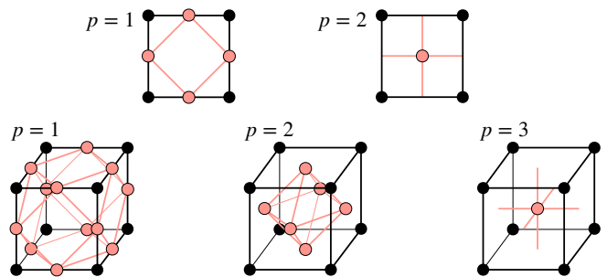
FIG. 15. The p -cells of the d -dimensional cubic lattice are equivalently the 0-cells of another lattice. Shown here are examples of this equivalent lattice embedded in the conventional unit cell of the cubic lattice, drawn in pink and black, respectively, for (first row) d = 2 and (second row) d = 3 .
