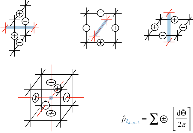
FIG. 11. Graphical representation of \hat{\rho}_{\hat{e}_{d-p-2}} (see Eq. (54)) in 3d space for (1st row) p = 0 and (2nd row) p = 1 . The \pm disks denote the sign in front of that \left[ \frac{d\tilde{\Theta}}{2\pi} \right] in the sum for \hat{\rho}_{\hat{e}_{d-p-2}} . The direct lattice is colored in black, the dual lattice is in red, and \hat{\rho}_{\hat{e}_{d-p-2}} is in blue.
