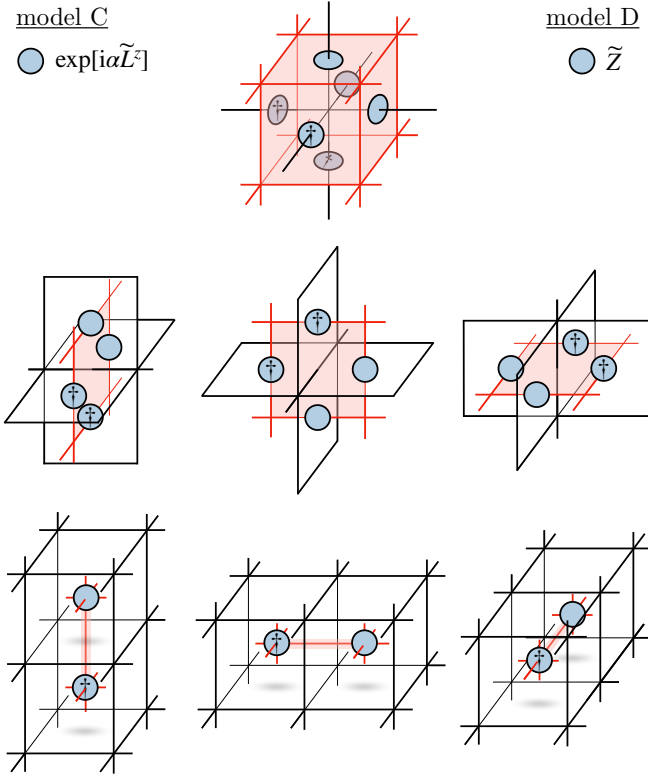
FIG. 9. Graphical representation of the emergent U(1)^{(p)} [ \mathbb{Z}_N^{(p)} ] symmetry operator Eq. (50) [(34)] in model C [D] acting on \partial\hat{c}_{d-p+1} in 3d space for (1st row) p = 1 , (2nd row) p = 2 , and (3rd row) p = 3 . The blue-colored disks denote the operator \tilde{L}_{c_p}^+ [ \tilde{X}_{c_p} ], the product of which yields the symmetry operator. Discs labeled by \dagger denote the hermitian conjugate of the operator and \hat{c}_{d-p+1} is colored red.
