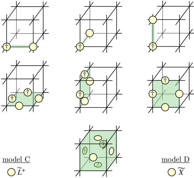
FIG. 8. Graphical representation of \widetilde{W}^\dagger(\partial c_{p+1}) for model C (Eq. (44)) and D (Eq. (28)) in 3d space for (1st row) p = 0 , (2nd row) p = 1 , and (3rd row) p = 2 . For model C (D), the yellow colored disks represent \widetilde{L}^+ ( \widetilde{X} ) operators, the product of which yields \widetilde{W}^\dagger(\partial c_{p+1}) . Discs labeled by \dagger denote the hermitian conjugate and c_{p+1} is colored green.
