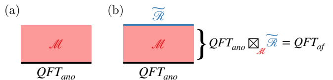
FIG. 3. (a) The low energy properties of QFT_{\text{ano}} ( QFT_{\text{af}} restricted to the \mathcal{R} -symmetric sub-Hilbert space) can be exactly simulated by a boundary of a topological order \mathcal{M} in one higher dimension. QFT_{\text{ano}} uniquely determines \mathcal{M} . (b) The low energy properties of QFT_{\text{af}} throughout all \mathcal{R} sectors can be simulated by including the boundary \tilde{\mathcal{R}} .
