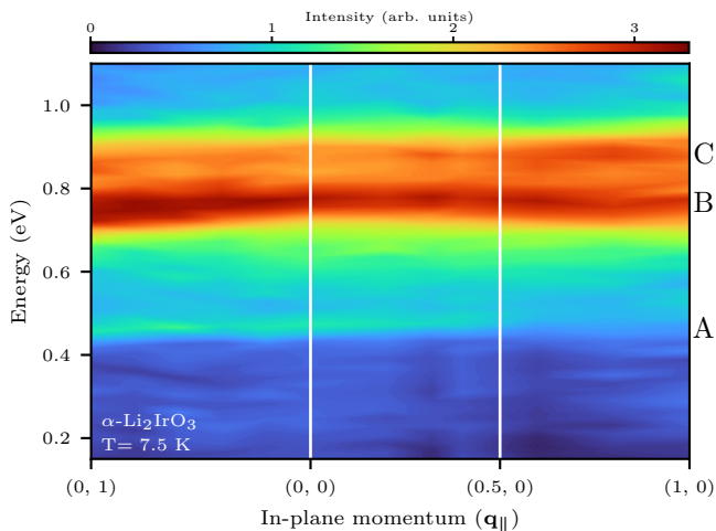
FIG. 2. In-plane momentum dependence of excitations in \alpha - \text{Li}_2\text{IrO}_3 at 7.5 K measured with Ir L_3 -edge RIXS. The main peaks are labelled from low to high energy as A, B, and C.
