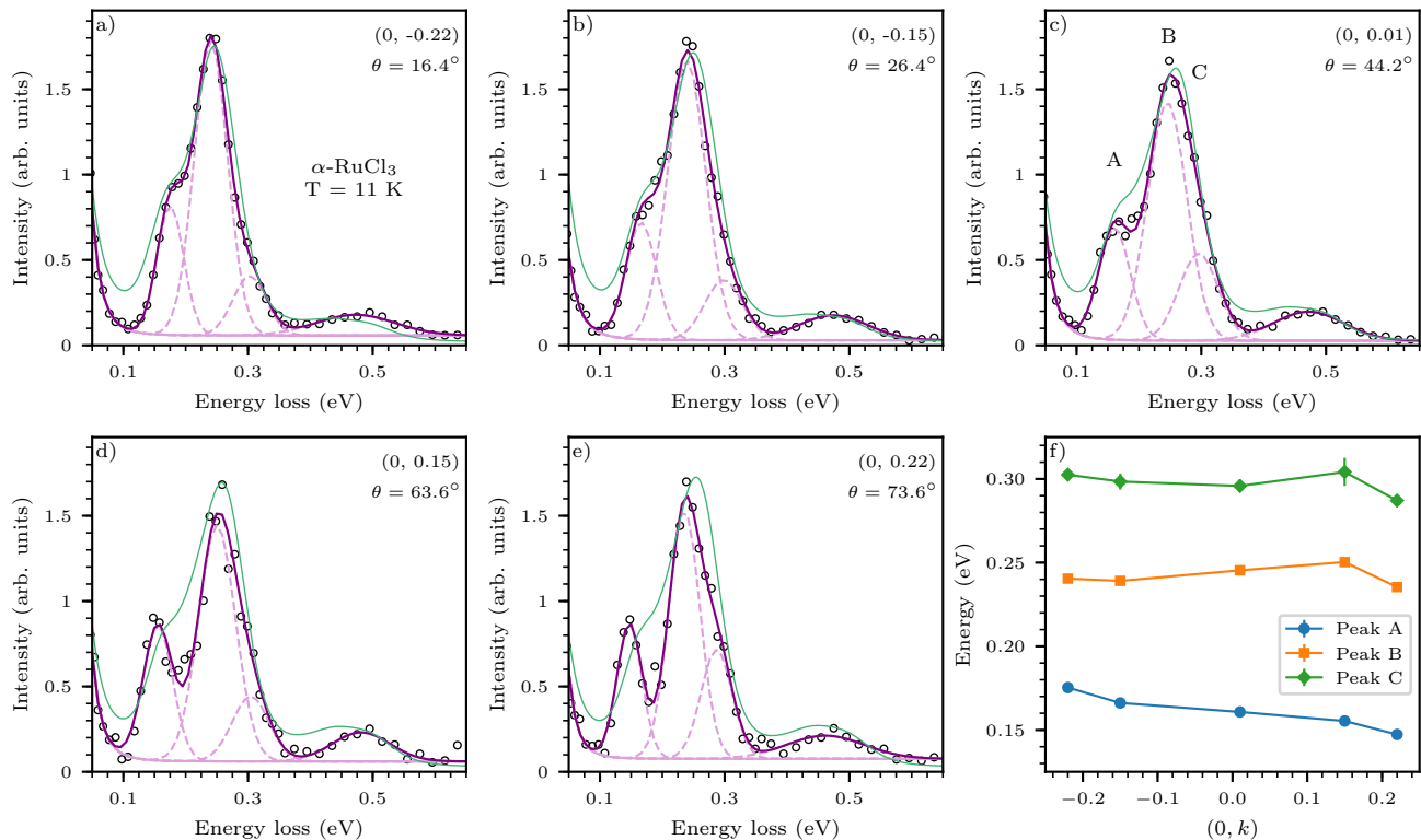
FIG. 3. Experimental Ru M_3 -edge RIXS data and fits of \alpha - \text{RuCl}_3 at 11 K compared to calculations. Spectra were taken with \mathbf{b}^* axis in scattering plane ( \phi = 90^\circ ) while varying \theta from grazing incidence (panel a) to grazing emission (panel e) with corresponding \mathbf{q}_{\parallel} and \theta shown in the top right corner of each panel. Data are shown as black circles and fits are shown as solid purple lines, with fit components as dashed purple lines: in particular peaks A, B, and C which are labelled in c), as well as an additional higher energy excitation. RIXS calculations are shown as green lines for \Delta_t < 0 . The momentum points and scattering geometry are decoupled in our calculations, therefore since all Ru M_3 -edge measurements are close to (0,0) we calculate the RIXS spectra at (0,0) while using the experimental \theta angle. The momentum dependence of the extracted peak positions are plotted in f).
