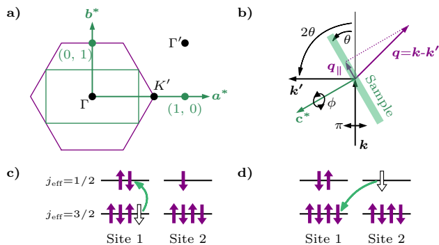
FIG. 1. a) In-plane reciprocal space showing hexagonal Brillouin zone (purple) and projection of C2/m Brillouin zone (green). The C2/m lattice is used throughout this paper and the projection of its \mathbf{a}^* = (h, 0) and \mathbf{b}^* = (0, k) axes are shown as green vectors. b) RIXS scattering plane used for experiments and calculations. Incoming x-rays with \pi polarization and momentum \mathbf{k} are scattered at 2\theta = 90^\circ with momentum \mathbf{k}' transferring \mathbf{q} = \mathbf{k} - \mathbf{k}' momentum to the sample (green bar). The sample is mounted with the honeycomb plane at an angle \theta leading to transferred in-plane momentum \mathbf{q}_{\parallel} . The azimuthal angle \phi rotates the sample around the \mathbf{c}^* axis, with \mathbf{a}^* ( \mathbf{b}^* ) in the scattering plane at \phi = 0^\circ ( \phi = 90^\circ ). c) & d) Schematic energy diagram of two excitation processes. Filled and unfilled arrows represent electrons and holes respectively, where up (down) arrows denote Kramer's doublet with positive (negative) eigenvalues of j_{\text{eff}}^z . See text for details.
