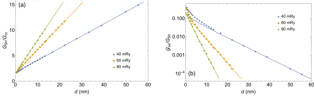
FIG. 7. Fits of the calculated (a) reduced resistance G_{SH}/G_{cc} and (b) the reduced spin conductance G_{ss}/G_{SH} as a function of the layer thickness d in bulk Pt calculated at E_F using the 16 \times 1 lateral supercell.
