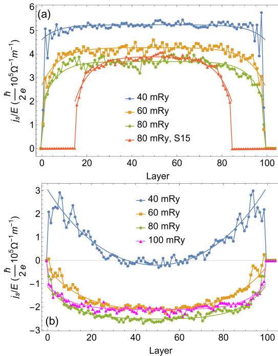
FIG. 3. Spin current in the Pt film expressed as shown in Eq. (12) in units of 10^5 \frac{\hbar}{2e} \Omega^{-1} \text{m}^{-1} . The calculated intrinsic spin-Hall conductivity of Pt reported in the literature is close to 4 \times 10^5 \frac{\hbar}{2e} \Omega^{-1} \text{m}^{-1} . The smooth lines are fits to Eq. (8) where l_{\text{sf}}^T is taken from the spin accumulation fits. (a) At E = E_F . (b) At E' = E_F - 2.72 eV.
