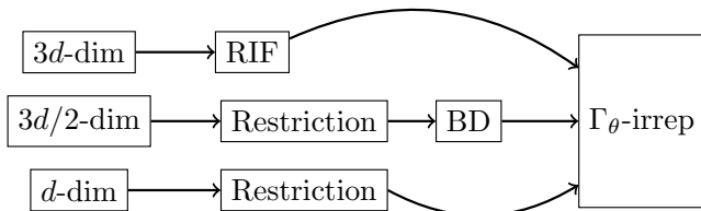
FIG. 1. Flowchart of computation of \Gamma_\theta -representations.
