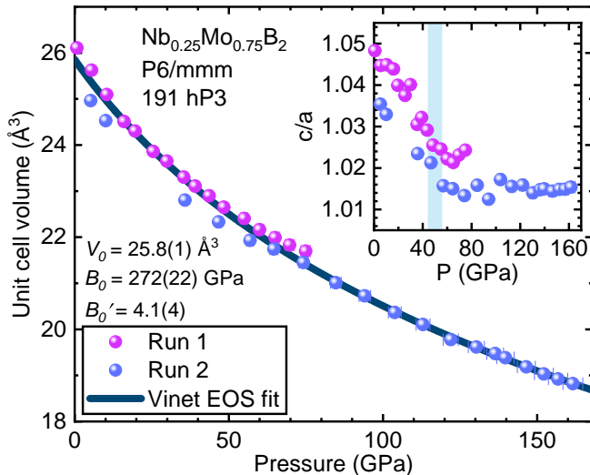
FIG. 5. P - V -isotherm of \text{Nb}_{0.25}\text{Mo}_{0.75}\text{B}_2 to 161 GPa at room temperature. Inset shows the c/a ratio versus pressure. There is a slope change above \sim 50 GPa marked by a light blue shaded area referring to the potential correlation with the slope change of T_c(P) in Fig. 3.
