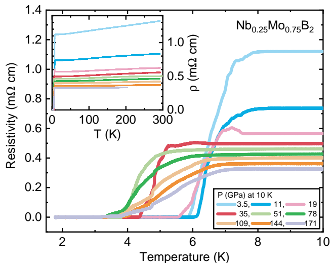
FIG. 2. Representative temperature-dependent resistivity curves of \text{Nb}_{0.25}\text{Mo}_{0.75}\text{B}_2 under pressure to 171 GPa (measured at 10 K) clearly showing the zero resistivity of superconducting transition between 1.8-10 K during each warming cycle. Inset shows the full 1.8-292 K temperature range studied.
