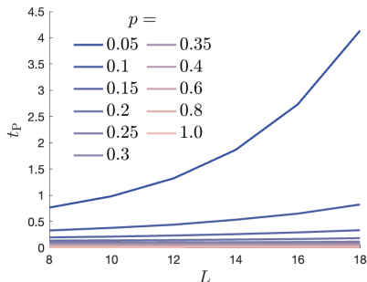
Figure 3: Qualitative comparison of the purification time’s growth with L at different p values. For p < p_c , the purification time diverges rapidly with system size in a manner consistent with exponential.
