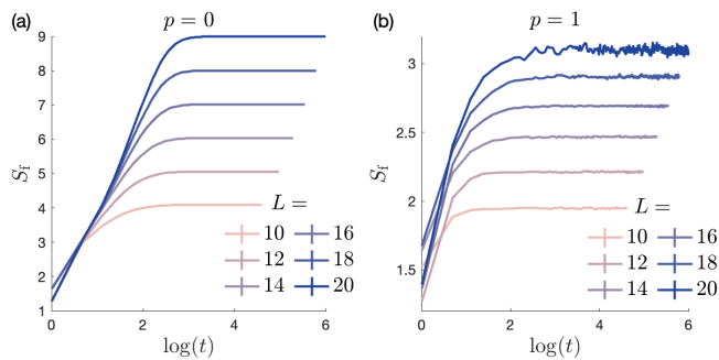
Figure 8: The bipartite entanglement entropy saturates after L^2 time steps. At the extreme p values p = 0, 1 , S_f quits changing (to within minor fluctuations).
