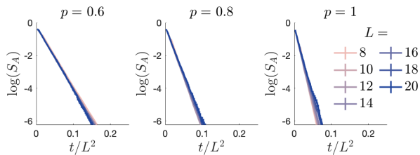
Figure 7: The purification time still reveals a z = 2 phase for p > 0.4 . The entropy S_A quantifies the ancilla qubit’s entanglement with the system. We plot \log(S_A) for clarity, as S_A decays exponentially. t/L^2 runs along the x -axis to demonstrate the existence of a phase in which the system purifies over a time scale t_P \sim L^2 . We used 30 000 samples when L = 8 to 16; 10 000 samples when L = 18 ; and 1 500 samples when L = 20 . The y -axis’s lower limit is \log(10^{-3}) \approx -6.91 .
