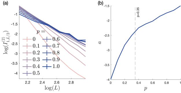
Figure 12: Mutual information at antipodal sites.
