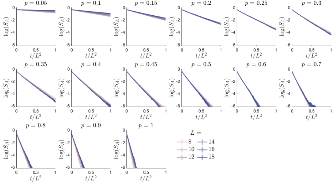
Figure 10: In the critical phase, the numerics are consistent with a \sim L^2 sharpening time scale. The entropy S_A quantifies the ancilla qubit’s entanglement with the system. We plot \log(S_A) for clarity, as S_A decays exponentially. t/L^2 runs along the x -axis to demonstrate the numerics are consistent with a \sim L^2 sharpening time scale. We used 30 000 samples when L = 8 to 14; and 10 000 samples when L = 16 to L = 18 . The y -axis’s lower limit is \log(10^{-3}) \approx -6.91 .
