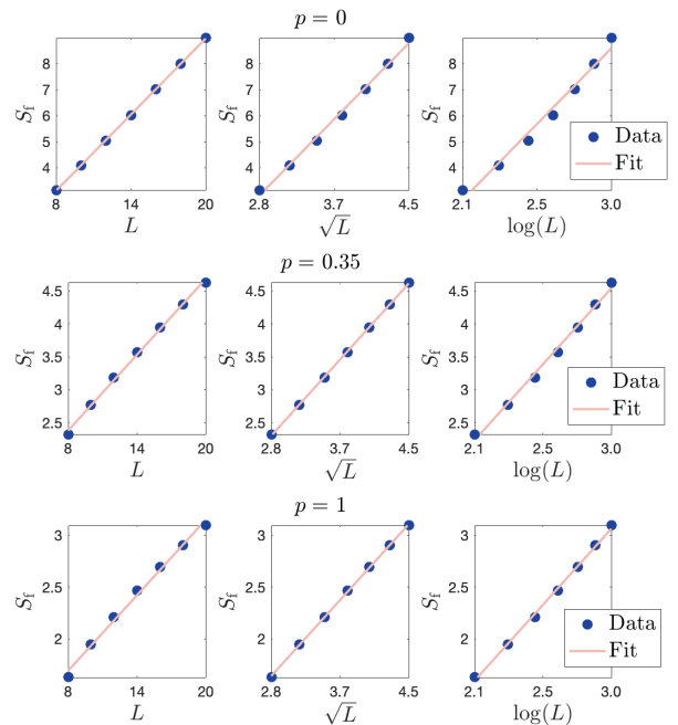
Figure 9: Long-time bipartite entanglement entropy vs. system size. At p = 0 , S_f \sim L , signaling a volume law. At p = 1 , the entropy scales logarithmically or as a small power law: S_f \sim \log(L) , or S_f \sim \sqrt{L} .
