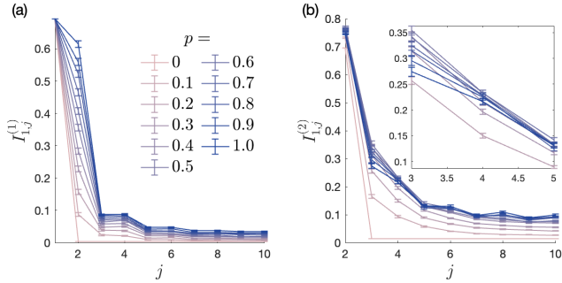
Figure 11: Mutual information between sites. The mutual information between (a) sites 1 and j decays more quickly than between (b) sites (1, 2) and (j, j + 1) . The inset highlights how I_{j,k}^{(2)} increases and then decreases as p grows, for some j . The errorbars represent one standard deviation.
