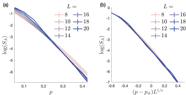
Figure 5: Evidence of spin-sharpening transition. The entropy S_A quantifies the ancilla qubit’s entanglement with the system. Different curves correspond to different system sizes L . (a) The curves’ crossing at p \approx 0.28 indicates a phase transition. (b) We identify a finite-size collapse using \nu = 3.0 and p_{\#} = 0.28 .
