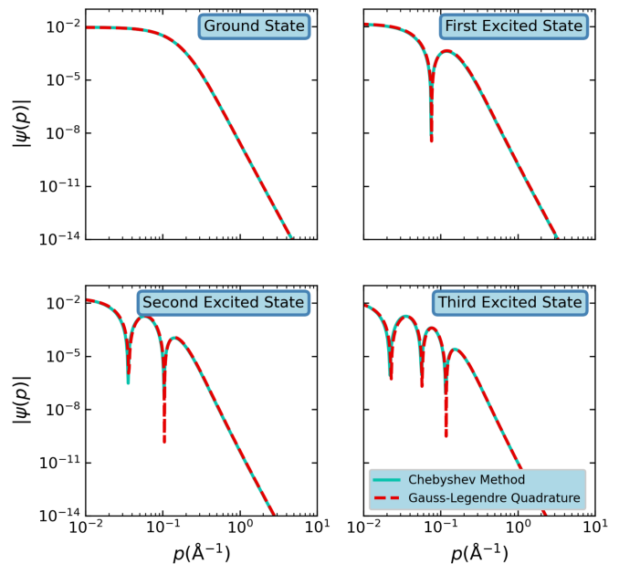
FIG. 10: (Color online) Comparison of wave functions obtained via (dashed red curves) the Gauss-Legendre quadrature method and (solid cyan curves) the Chebyshev method for the first four states of the MoS 2 exciton using the RK potential. \psi_i(p) is the i -th excited state for the s -wave. Note that the y -axis is in log scale, and the number of peaks represents the number of nodes in the excitonic wave function.
