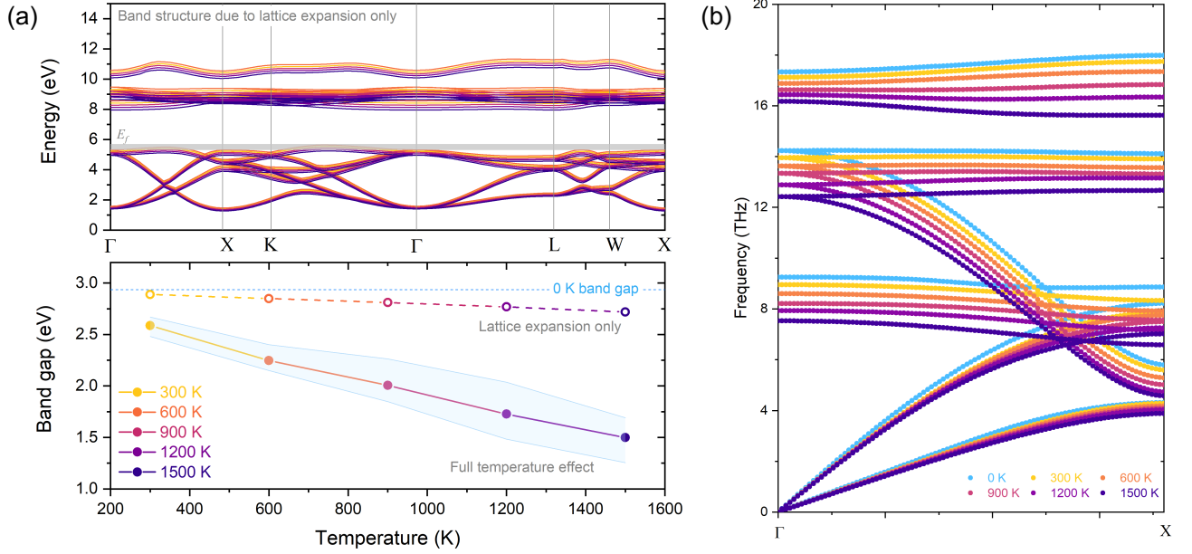
FIG. 1. Temperature-dependent band structure and phonon dispersions. (a) Band structure with lattice expansion only (top panel), and the band gap as a function of temperature (bottom panel) when only lattice expansion is considered (dashed line) or dynamical effect is included (solid line). In top panel, the band structure at each T is obtained by non-self-consistent DFT calculations at relaxed unit cell structure that comes from AIMD simulations under NPT ensemble. In the bottom panel, data points of full effect are the averaged band gap values calculated from 10 snapshots in AIMD simulations and the shaded area is the span of those 10 gap energies at each T . DFT band gap at 0 K is shown in blue dotted vertical line as a reference. (b) Phonon dispersions at finite T . All phonon energies are reduced with rising temperatures. Longitudinal and transverse optical phonon splitting is treated by considering long-range interactions using Born effective charge calculated by DFPT [27].
