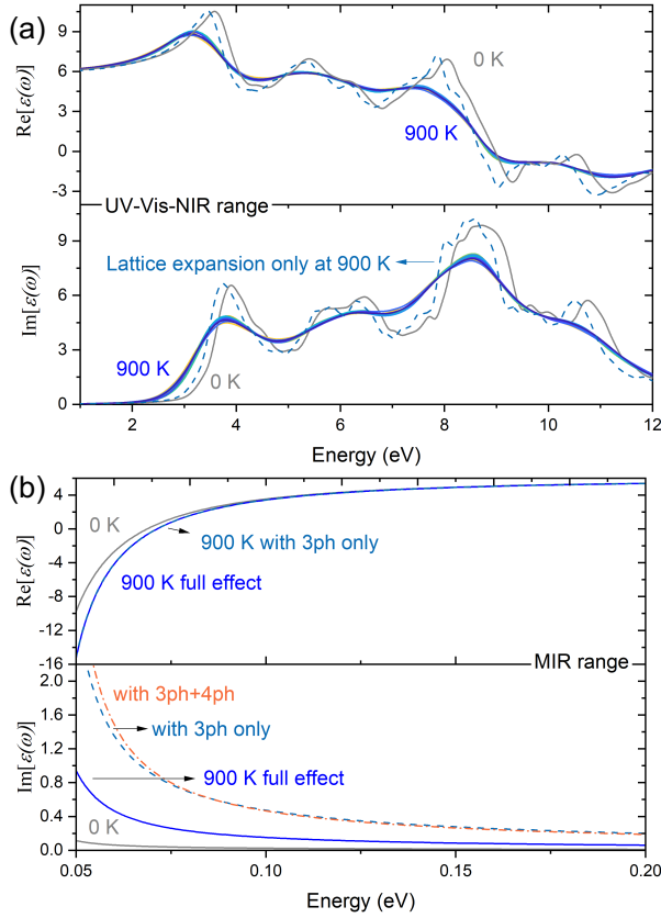
FIG. 2. Dielectric function \epsilon(\omega) at 0 K (grey lines) and 900 K (blue lines). (a) \epsilon(\omega) from electronic transition in UV-Vis-NIR range. Each colored solid line represents the dielectric function for one snapshot structure in AIMD simulations. Dashed lines are \epsilon(\omega) calculated on relaxed structure at 900 K. (b) \epsilon(\omega) from phonon resonances in MIR range. Damping factor for 0 K is approximated by scattering rates at 5 K. Dashed cyan lines represent \epsilon(\omega) with only 3ph scattering included. Dash-dot orange line represents \epsilon(\omega) with 3ph+4ph scattering included. Solid lines represent \epsilon(\omega) with both 3ph and 4ph scattering and phonon renormalization. In the upper panel of (b), dashed line nearly overlaps with solid line.
