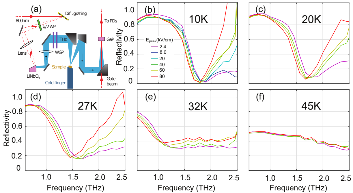
FIG. 2. \text{La}_{1.85}\text{Sr}_{0.15}\text{CuO}_4 c-axis THz reflectivity. (a) Schematic of experimental setup. Panels (b)-(f) show the reflectivity taken at temperatures 10 K, 20 K, 27 K, 32 K, and 45 K respectively. At each temperature, the reflectivity was measured for fields ranging from 2.4 – 80 kV/cm as indicated in the legend.
