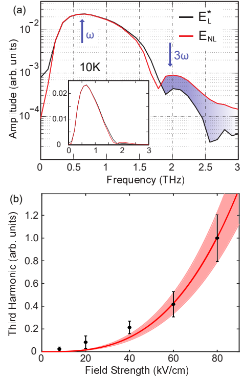
FIG. 3. Third harmonic generation from c -axis LSCO at 10K. (a) Linear (black) and nonlinear (red) spectral amplitude of the THz pulses reflected from the sample. The nonlinear spectrum is at the maximum field strength of \sim 80 kV/cm, and the linear spectrum is at the minimum field strength (renormalized as explained in the text). The shaded region in blue is the spectral content attributed to third harmonic generation. The inset contains a plot of the spectral amplitudes with a linear y-axis. (b) Third harmonic generation as a function of incident THz field strength at 10K. Each data point is from integrating Eq. 1 over the third harmonic region. The red line is a cubic polynomial fit, and the shaded area is bounded by cubic fits of the data including the upper and lower bounds of the data including the error bars.
