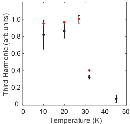
FIG. 4. Magnitude of c -axis THG from LSCO versus temperature. All data points were taken with maximum field strengths of 80 kV/cm. The black circles are experimental data and the red circles are calculations as described in the text. The experimental data and calculations are normalized to the maximum value, which occurs at 27K in both experiment and simulation.
