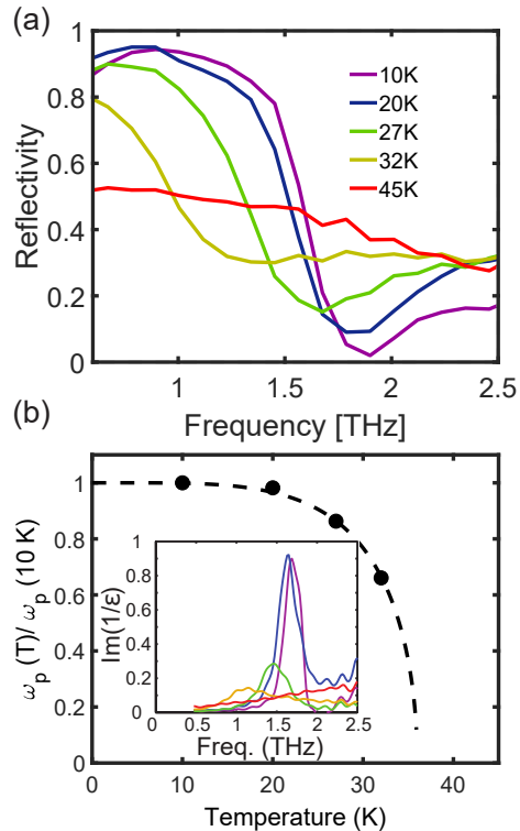
FIG. 1. (a) Low field c-axis reflectivity of \text{La}_{1.85}\text{Sr}_{0.15}\text{CuO}_4 at several temperatures. At 10K, \omega_p is \sim 1.7 THz. (b) Temperature dependence of \omega_p below T_c normalized to the low temperature measurement \omega_p(T = 10 \text{ K}) . The dashed line is a fit to a BCS-like order parameter temperature dependence, as described further in the text. The inset shows the (normalized) loss function, -\text{Im}(1/\epsilon) , using the same legend in panel (a).
