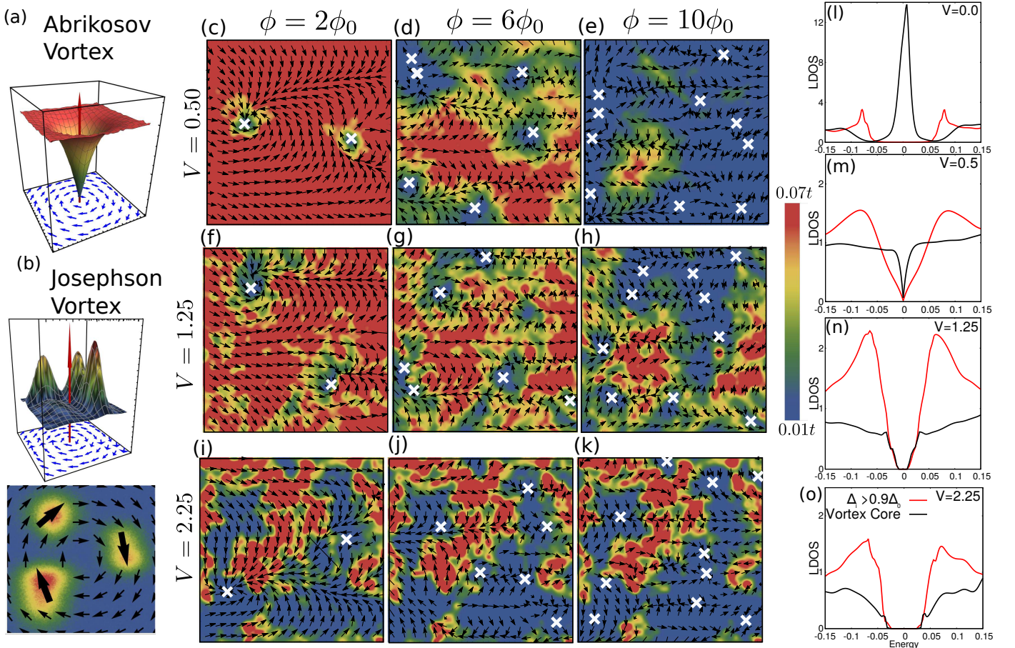
FIG. 2: Crossover from Abrikosov to Josephson vortices with increasing disorder: Panel (a): Schematic plot of an Abrikosov vortex showing the suppression of the pairing amplitude and the curling of the phase around the vortex core. Panel (b): Schematic plot of a Josephson vortex centered in the non-SC region surrounded by 3 SC-islands with finite pairing amplitude \Delta . Magnetic field shown by red vertical arrows in (a) and (b). The spatial color-density map of the superconducting pairing amplitude (in one unit cell; see SM) with H increasing from left to right along each row for weak V = 0.5 (panels (c-e) in the top row), moderate V = 1.25 (panels (f-h) in the middle row) and strong V = 2.25 (panels (i-k) in the bottom row) disorder strengths. The phase of order parameter is superimposed on the amplitude map by tiny arrows. Panels (l-o): LDOS [47] at vortex core (black) and away from core (red) for weak H , with increasing disorder.
