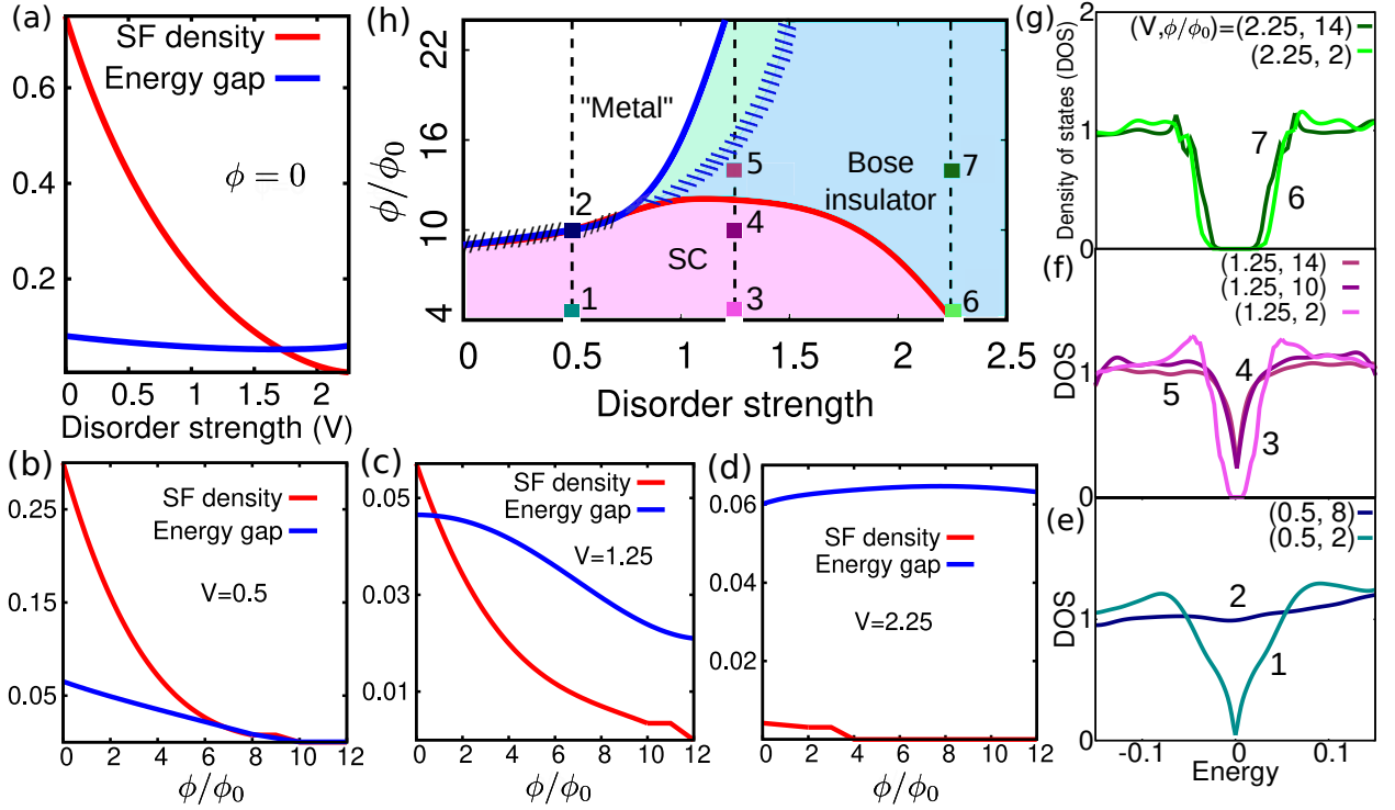
FIG. 3: Phase diagram of the 2D superconductor in the disorder V - magnetic field H plane. Panels (a-d): evolution of superfluid stiffness D_s , including harmonic quantum phase fluctuations [53–55] (See SM) and single-particle spectral gap E_g for H = 0 vs. disorder V [weak ( V = 0.5 ), moderate ( V = 1.25 ) and strong ( V = 2.25 )]. Panels (e-g): average DOS, N(\omega) for different H and V . The magnetic field H is in units of \phi , the number of SC flux quanta penetrating a 36 \times 36 magnetic unit cell. Panel (h): Phase boundaries in the V - H plane – critical fields obtained from vanishing of D_s (red trace) and vanishing of E_g (blue trace). The phase diagram features three distinct regions: (I) SC ( E_g \neq 0 and D_s \neq 0 ); (II) fermi metal or gapless fermionic Anderson insulator 56) ( E_g = 0 and D_s = 0 ); and (III) Bose insulator ( D_s = 0 , E_g \neq 0 ). The region III is further divided by a hashed line where the ‘two-particle’ gap in \sigma(\omega) disappears.
