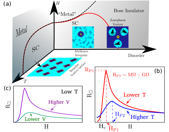
FIG. 1: (a) Schematic Phase diagram of a type II superconductor along the magnetic field ( H ), temperature ( T ), and disorder ( V ) axes reveals 3 phases: SC with single particle gap E_g \neq 0 and superfluid stiffness D_s \neq 0 ; fermionic metal E_g = 0 and D_s = 0 ; and Bose insulator E_g \neq 0 and D_s = 0 . The vortices change character from Abrikosov-type with metallic cores to Josephson-type with insulating cores as V is increases. (b,c) illustrates the experimental puzzles in the magnetoresistance (MR) which rises sharply beyond the SIT at H_c by orders of magnitude [23–31], whose explanations emerge naturally from our phase-diagram.
