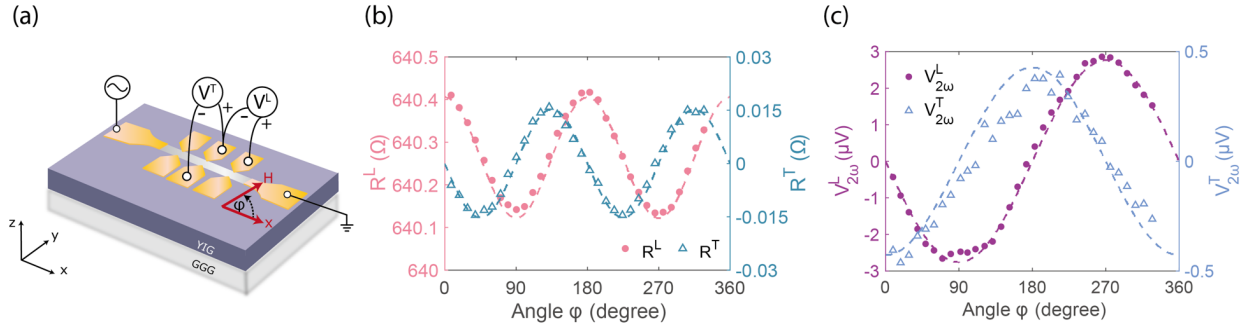
FIG. 1. (a) Schematic illustration of the longitudinal resistance ( R^L ) and Hall resistance ( R^T ) measurements with two lock-in amplifiers. The frequency and root-mean square (rms) amplitude of the sinusoidal excitation current are \omega/2\pi = 1017.1 Hz and I_\omega = 1 mA, respectively. The H field is -20 mT. (b) Angular dependence of R^L and R^T measured as the ratios between the corresponding in-phase (X) 1\omega voltages ( V_{\omega,X}^L and V_{\omega,X}^T ) and I_\omega . (c) Angular dependence of the out-of-phase (Y), 2\omega components of the longitudinal ( V_{2\omega,Y}^L ) and transverse ( V_{2\omega,Y}^T ) voltages. The lines are model fitting to the measurement data (symbols).
