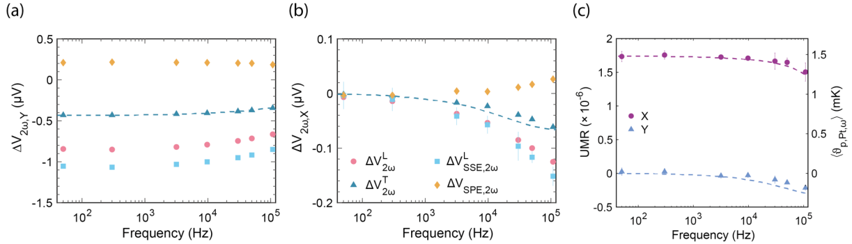
FIG. 3. The out-of-phase (a) and in-phase (b) components of the \Delta V_{2\omega} (symbols) as a function of the frequency of the current modulation at 1.08 mA amplitude in the Pt line. In panels (a) and (b), \Delta V_{2\omega}^T are compared with the analytical solutions with \lambda = 830 nm, l_{mp} = 250 nm, \kappa_M = 0.1 Wm ^{-1} K ^{-1} , \sigma_m = 1.85 \times 10^6 Sm ^{-1} , S_m = 63.5 \mu VK ^{-1} , and S_s = 65.5 \mu VK ^{-1} . The legend in panel (b) is for panel (a) and (b). The error bars indicate the statistical uncertainty with 95% confidence. (c) UMR (left axis) and equivalent Pt phonon temperature modulation (right axis) due to the SPE at \varphi = -90^\circ as a function of the current frequency at 4.7 \times 10^9 A m ^{-2} current density. The dashed lines in panel (c) are obtained from the analytical solutions with the same parameters as those in (a) except that S_m = 45.0 \mu VK ^{-1} and S_s = 168.0 \mu VK ^{-1} .
