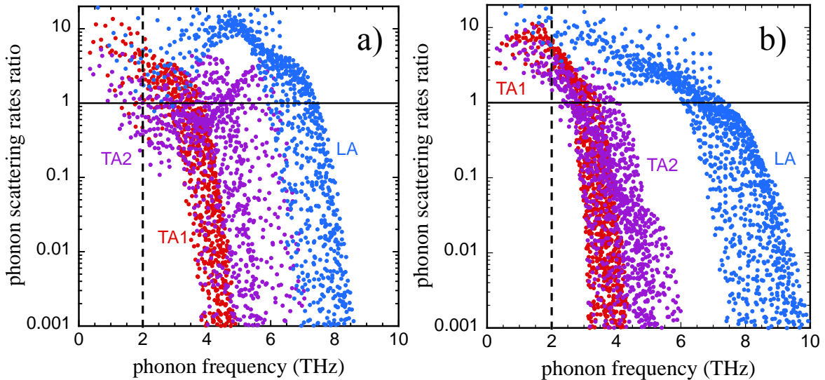
Figure 3: a) Ratio of phonon-hole scattering rates to three-phonon scattering rates in BAs for hole density, p=10^{21} \text{ cm}^{-3} and at 300 K; b) Same for Si. Ratios are broken down by acoustic phonon branches. Red: transverse acoustic 1 (TA1); purple: transverse acoustic 2 (TA2); blue: longitudinal acoustic (LA). Vertical dashed black lines separate regions of low and high frequency phonons.
