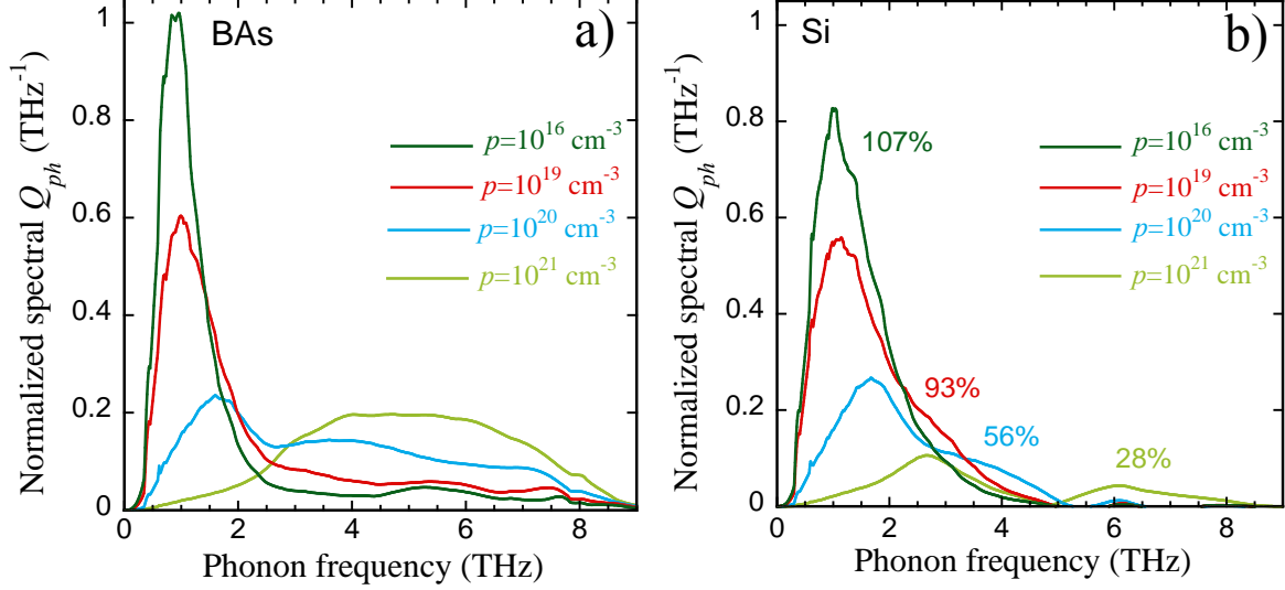
Figure 2: Normalized spectral phonon contributions to the room temperature Q_{ph} . a) BAs; b) Si; for four hole densities: p=10^{16} \text{ cm}^{-3} , 10^{19} \text{ cm}^{-3} , 10^{20} \text{ cm}^{-3} , and 10^{21} \text{ cm}^{-3} . The percentages in Fig. 2 b) indicate the scaling factor, Q_{ph}(\text{Si})/Q_{ph}(\text{BAs}) , weighting the Si contributions relative to those in BAs.
