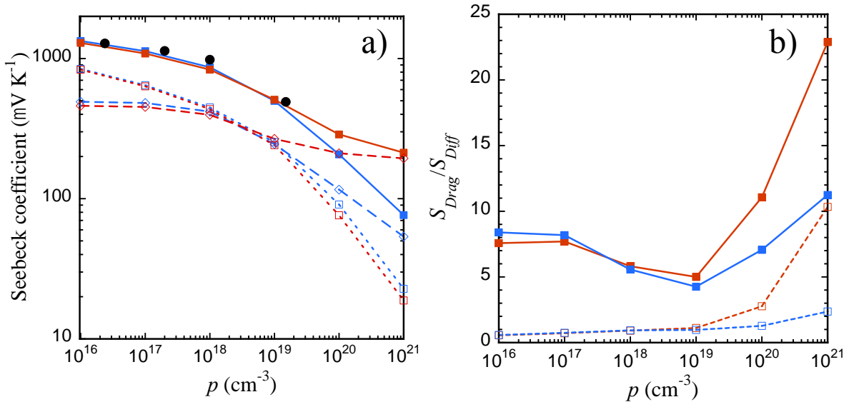
Figure 1: Seebeck coefficients for BAs and Si as a function of hole density, p , at 300 K. a) BAs: solid red curve; Si: solid blue curve. Black circles are measured data for Si [6]. Short dashed and long dashed curves give S_{diff} and S_{drag} ; b) Ratio of S_{drag} to S_{diff} for BAs (red) and Si (blue) at 300 K (dashed) and at 100 K (solid).
