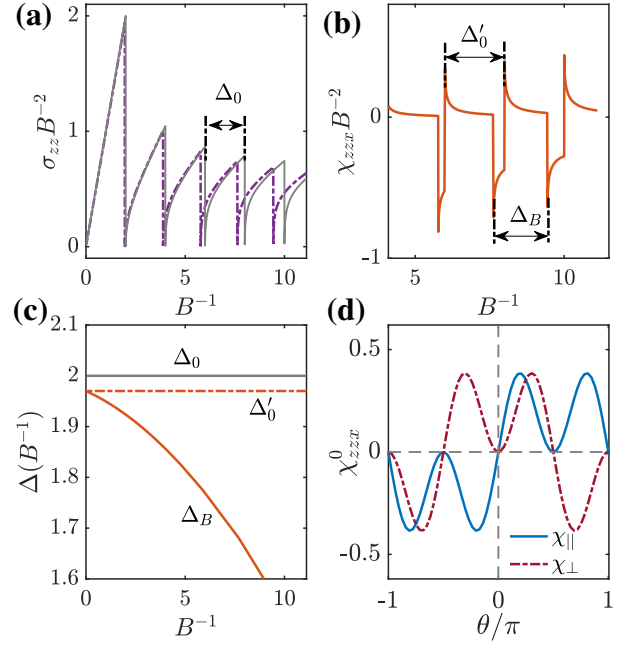
FIG. 3. (Color online) Periodic oscillations in B^{-1} of the linear ( \sigma_{zz} ) and nonlinear conductivity ( \chi_{zzx} ) in panel (a) and (b), respectively. Note that the additional \beta_x^E does not make big difference on the magnitudes of \sigma_{zz} . The constant periods \Delta_0, \Delta'_0 and the magnetic field dependent \Delta_B are compared in panel (c). Here, E_F = v_F \sqrt{e\hbar} (= 1\hbar\omega_c|_{B=1}) is taken. Panel (d) presents the angular dependencies of the longitudinal ( \chi_{\parallel} ) and transverse ( \chi_{\perp} ) components of the magneto conductivity tensor, here \theta = \langle \mathbf{E}, \mathbf{B} \rangle as shown in Fig. 1.
