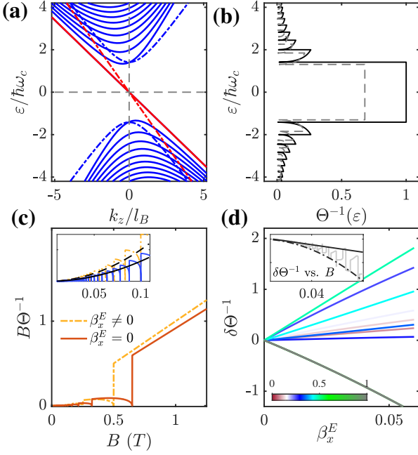
FIG. 2. (Color online) (a) Landau levels (LLs) projected in the k_y = 0 plane for Weyl node s = +1 , where the solid (dashed) lines represent the LLs of a tilted (non-tilted) Weyl node. Panel (b) presents the oscillating DOSs \Theta^{-1} as function of Fermi energy. The dashed (solid) curves imply for the case with \beta_s \neq 0 i.e. \beta_x^E = 0.1, \beta_y^w = 0.1 ( \beta_s = 0 , i.e. \beta_x^E = \beta_y^w = 0 ). To better reveal the modification, here a finite w_z = 0.3 is taken for the case with \beta_s \neq 0 . Panel (c) plots B\Theta^{-1} as function of B , where the inset shows the quadratic-in- B dependence in the weak- B limit. (d) depicts the linear dependency of \delta\Theta^{-1} on \beta_x^E at various magnetic field strengths (indicated by the color scale). The inset shows \delta\Theta^{-1} \propto B in the weak- B limit.
