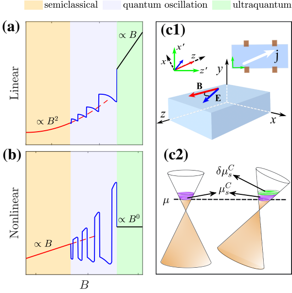
FIG. 1. (Color online) The phenomenological magnetic field dependence of the linear and nonlinear magneto planar conductivity induced by chiral anomaly (CA) in WSMs are shown in (a) and (b) respectively, for three transport regimes. Panel (c1) presents the geometry of a crossed fields lying in the x-z -plane, and the schematic setup for experimental probing ( top right , inset) along with the possible coordinate systems ( top left , inset). (d) shows the CA-induced chiral chemical potential (purple, \mu_s^C ) and its deviation (green, \delta\mu_s^C ) for a single Weyl cone.
