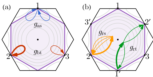
FIG. 4. Scattering of fermions between Van Hove singularities (VHSs) by (a) density-density interactions g_{bt} (red), g_{as} (blue) and (b) non-vanishing processes g_{rs} (yellow), g_{rt} (green) of H_{\text{int, CF}} . Thin (or thick) arrows correspond to A -type (or B -type) fermions.
