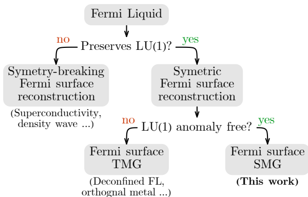
FIG. 6. Classification of Fermi surface reconstruction mechanisms, based on the LU(1) loop group symmetry. Symmetric Fermi surface reconstruction (SFSR) contains two broad classes: (1) Fermi surface symmetric mass generation (SMG) if the total Fermi surface anomaly is canceled. (2) Fermi surface topological mass generation (TMG) if the total Fermi surface anomaly is matched by topological order with low energy topological field theory.
