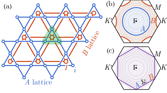
FIG. 3. (a) In the real space, we design the overlapping Kagome ( A ) and triangular ( B ) lattices. The green triangle marks out the unit cell. In the momentum k space, we draw many contours to represent various equal energy curves of the energy band, at different filling levels (equally spaced by 1/8 filling fraction). We illustrate the A -type (in blue) and B -type (in red) Fermi surfaces (b) at a general filling such as \nu_A = 3/8 and \nu_B = 7/8 (= -1/8) , or (c) at a special filling \nu_A = \nu_B = 3/4 (= -1/4) where the Fermi surfaces coincide.
