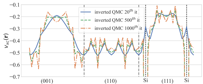
FIG. 15. Exchange-correlation potentials obtained by inversion of the QMC density of bulk silicon, at three different iteration steps. All three potentials yield a very similar, accurate density. The MeAPE of the density is 0.04% at i = 20 , 0.02% at i = 500 , and the same value at i = 1000 . For the MaAPE, we get 0.38% at i = 20 , 0.21% at i = 500 , and 0.18% at i = 1000 .
