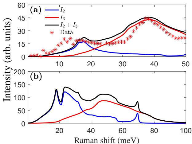
FIG. 4. Unpolarized Raman spectrum of \alpha -SrCr 2 O 4 in (a) and \alpha -CaCr 2 O 4 in (b). (a) The blue line is the bimagnon Raman spectrum I_2 . The red line corresponds to the trimagnon Raman spectrum I_3 . The black line is the total Raman spectrum I_2 + I_3 . Both I_2 and I_3 are the results of our fitting procedure. We report a new set of interaction parameters, \mathcal{P}_6 in Table I, generated from our model and based on the experimental data reported in Ref. 29 (displayed as red asteriks). The calculation utilizes p_1 = p_2 = p_3 = 1 , and p_4 = 0.42 . (b) Predicted unpolarized Raman spectrum of \alpha -CaCr 2 O 4 . The spectrum was calculated based on the experimental parameter set \mathcal{P}_5 reported in Ref. 21. For \alpha -CaCr 2 O 4 , I_2 and I_3 were computed with p_1 = p_2 = p_3 = p_4 = 1 .
