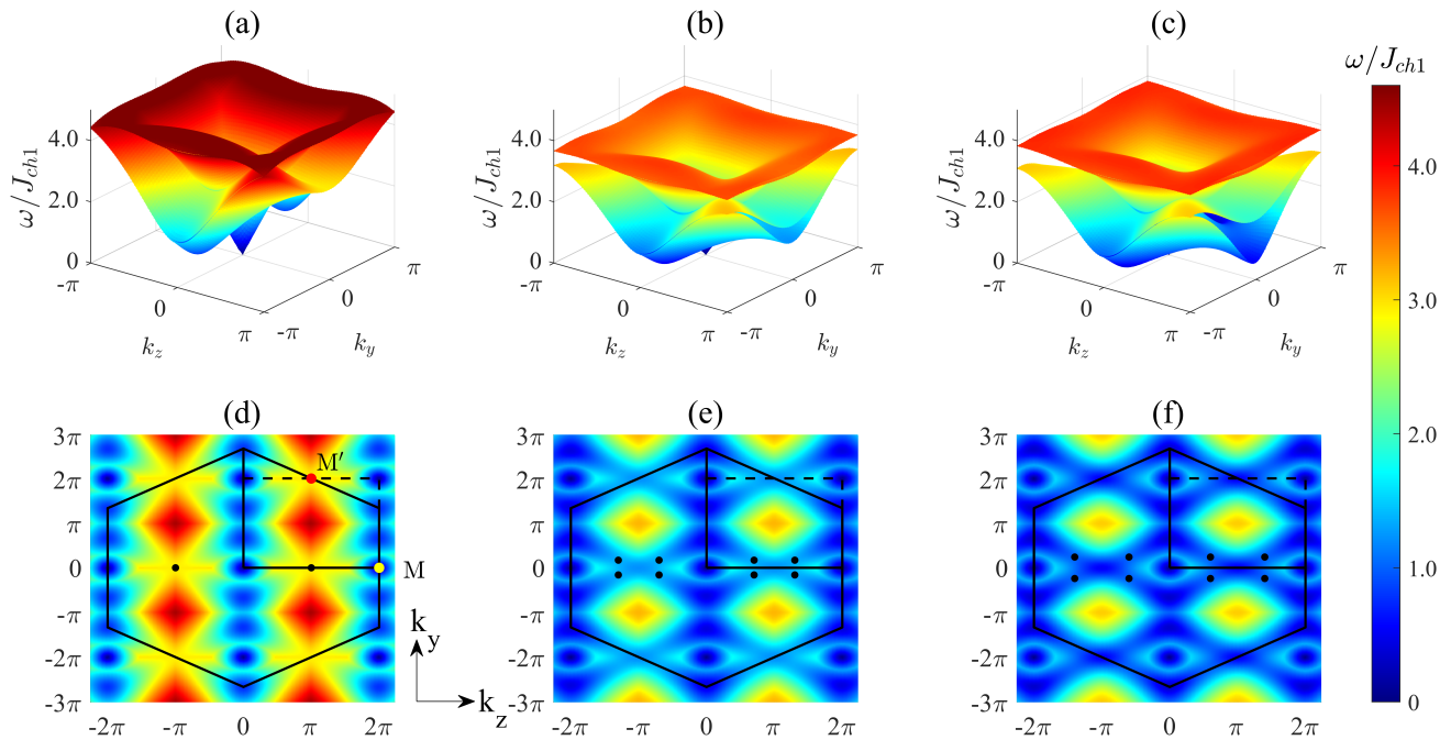
FIG. 2. Spin wave dispersion of the triangular lattice antiferromagnet. (a) - (c) are spin wave dispersions for parameter sets \mathcal{P}_1 , \mathcal{P}_4 , and \mathcal{P}_5 , respectively. There are four branches of energy for each parameter set as the unit cell contains four sublattices. (d) - (f) are one of the four energy branches with the lowest energy which correspond to (a) - (c). M(0, 0, 2\pi) and M'(0, \pi, 2\pi) are the rotonlike points of the undistorted triangular antiferromagnet for \mathcal{P}_1 . The roton minimum energy can be observed in rotonlike points indicated by the black dots. We observe the roton energy minimum at different spin wave dispersion branches for various parameter sets, see Table I. Distortion results in M' becoming the only rotonlike point which split into four different points in the spin wave dispersion. Enhanced distortion spreads the split rotonlike points (indicated by the eight black dots in panel (e)) into four different directions in momentum space (see panel (f)).
