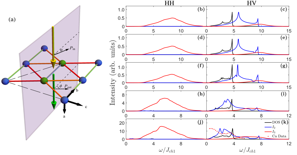
FIG. 3. (a) Raman scattering geometry. Incident light is always assumed to be along the a axis. The angle \theta and \phi are defined as displayed in the figure. (b)-(k) present the polarized bimagnon I_2(\omega, \theta, \phi) and the trimagnon I_3(\omega, \theta, \phi) Raman spectra. Each row refers to the parameter choice \mathcal{P}_i with i = 1, \dots, 5 , respectively (see Table I). The first column represents HH polarization with (\theta, \phi) = (0, 0) . The second column is HV polarization with (\theta, \phi) = (0, \frac{\pi}{2}) . All the calculated Raman intensities are computed by applying p_1 = p_2 = p_3 = p_4 = 1 and a small broadening parameter 0^+ = 0.02 meV. The black solid line is single-magnon density of states. Red dots are extracted using WebPlotDigitizer [51] from the Raman experiment in circular RL polarization reported for \alpha - \text{CaCr}_2\text{O}_4 in Ref. 28.
