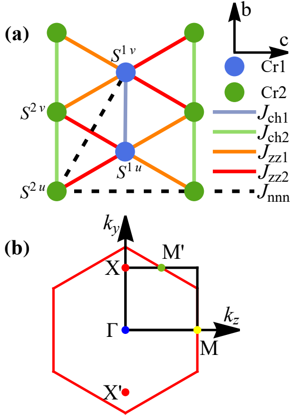
FIG. 1. (a) Unit cell of \alpha -SrCr 2 O 4 [31] and \alpha -CaCr 2 O 4 [20]. The positions of the four Cr 3+ ions are (0, 0, 0), (0, 0.5, 0), (0, 0.25, 0.5 - 0.01d), and (0, 0.75, 0.5 + 0.01d) with site indices denoted by i \in \{2u, 2v, 1u, 1v\} , where d is the lattice distortion parameter. The two inequivalent Cr 3+ ions are shown as blue Cr1 and green Cr2 symbols. The spins are labeled as \mathbf{S}^{1u} , \mathbf{S}^{1v} , \mathbf{S}^{2u} and \mathbf{S}^{2v} . (b) The black box is the first Brillouin Zone (BZ) of the unit cell with four spins. The red hexagon is the first BZ of the undistorted TLAF which contains only one spin in the unit cell. The high symmetry points \Gamma , M, M', X, and X' are shown in the BZ. The wave vectors are denoted by k_y and k_z .
