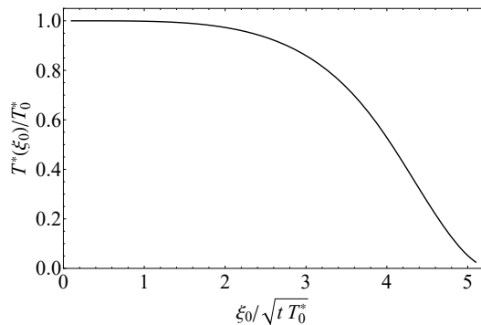
FIG. 6. Suppression of the time-reversal symmetry breaking temperature T^* by the deviations from circularly-symmetric Fermi surface (Eq. (9)) characterized by the parameter \xi_0 = \frac{v_F^{(2)}t\theta_{\text{MA}}}{2v_\Delta} .
