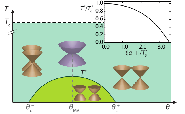
FIG. 5. Phase diagram of the secondary time-reversal symmetry breaking superconducting order induced by the quasi-particle interactions near the magic angle. Its onset temperature T^* reaches its maximal value T_0^* at the magic angle and is suppressed as the deviation |\theta - \theta_{MA}| grows, vanishing at \theta_c^\pm = \theta_{MA} \pm 2\pi e^{-\gamma} \frac{\theta_{MA} T_0^*}{t} . The band structure schematics represent the qualitative form of the quasiparticle spectrum in each region (cf. Fig. 3). Inset shows the numerical solution for T^*(\theta) as a function of the dimensionless twist parameter t|\alpha - 1|/T_0^* . Here, T_0^* \ll T_c is assumed; see text for the discussion of the additional effects of temperature.
