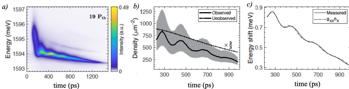
FIG. 5. a) Time-resolved energy spectrum of a polariton condensate in a one-dimensional trap, recorded with a streak camera. The oscillations arise because the polaritons at late times are effectively in a macroscopic, one-dimensional harmonic potential. b) Solid line: Measured density of the polaritons at the potential energy minimum (gray area gives the uncertainty). Dashed line: estimated exciton reservoir density. c) Comparison of the measured energy shift of the lower polariton line and the predicted energy shift deduced from the density data of (b). The constant of proportionality gives the interaction constant g . From Ref. 33.
