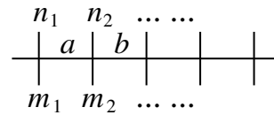
FIG. 2. The matrix elements of a string-like tensor network operator, O_{m_1, m_2, \dots; n_1, n_2, \dots} , can be given by a contraction of rank-4 tensors T_{n_2, m_2, a, b} , etc. Each tensor is represented by a vertex, where the legs of the vertex correspond to the indices of the tensor. The connected legs have the same index and is summed over (which correspond to the tensor contraction). This is just one representation of tensor network operator.
