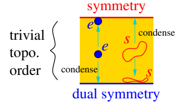
FIG. 20. All the non-trivial excitations in the bulk 2\mathcal{G}\text{au}_{\mathbb{Z}_2} , either condense on the 2\mathcal{R}\text{ep}_{\mathbb{Z}_2} -boundary ( s condense) or condense on the 2\mathcal{V}\text{ec}_{\mathbb{Z}_2} -boundary ( e condense). Thus the slab has no topological excitations and correspond to a trivial topological order.
