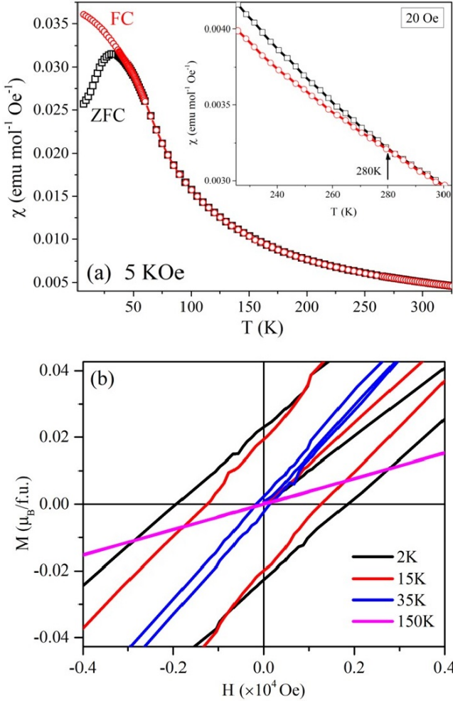
FIG. 3. Top : Temperature dependent dc Susceptibility ( \chi_{dc} ) measured at 5KOe showing bifurcation between ZFC and FC curves below 47K, Inset: \chi_{dc} measured at H = 20 Oe showing the separation of ZFC and FC curves at 280K, Bottom : M(H) curves showing small, but finite hysteresis below T_f indicating a weak FM contribution.
