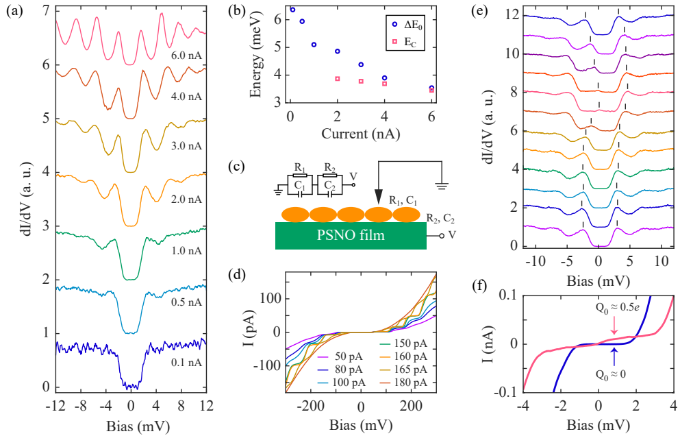
FIG. 4. (a) A series of dI/dV spectra on a 25.5-nm PSNO nanocluster as a function of tunneling current setpoints. The bias setpoints are stabilized at 12 mV. (b) The extract \Delta E_0 and E_C as a function of the current setpoints. (c) Schematic illustration of the DBTJ model on the PSNO surface and equivalent circuit of this structure. (d) A series of I - V curves measured on a 4.66-nm PSNO nanocluster at different tunneling current setpoints. The bias setpoints are fixed at 300 mV. (e) A series of dI/dV spectra (setpoints: V = 12 mV, I = 1.3 nA) acquired along a trajectory of 8.0 nm in an 18.1-nm PSNO nanocluster. (f) Comparison of I - V curves between Q_0 \approx 0 and Q_0 \approx 0.5e .
