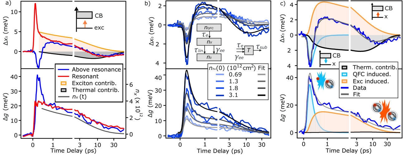
FIG. 2. a) Time-dependent exciton peak-shift ( \Delta x_0 ) and broadening ( \Delta g ) for above-resonance (blue) and resonant (red) pumping with an absorbed photon density n_{h\nu}(0) = 3.1 \cdot 10^{12} \text{ cm}^{-2} . binding energy reduction (orange solid) and temperature-induced (solid grey) contributions to resonant peak-shift dynamics. The time-dependent exciton density n_x(t) is displayed on the right axis of the bottom panel. b) Above-resonance pumping: time-dependent exciton peak-shift and broadening for different fluences with corresponding fit using Eq. 10 and Eq. 9. Inset: sketch of the three-level model. c) Top panel: Time-dependent exciton peak-shift for above-resonance pumping and corresponding fit with Eq. 10 (from Fig. 2.b)). Time-dependent contributions to the peak-shift originating from temperature increase (grey), QFC (light blue) and excitons (orange). Bottom panel: photoinduced broadening and respective fit with Eq. 9 from Fig. 2.b). Contribution to the broadening from QFC-exc (light blue) and exc-exc scattering (orange).
