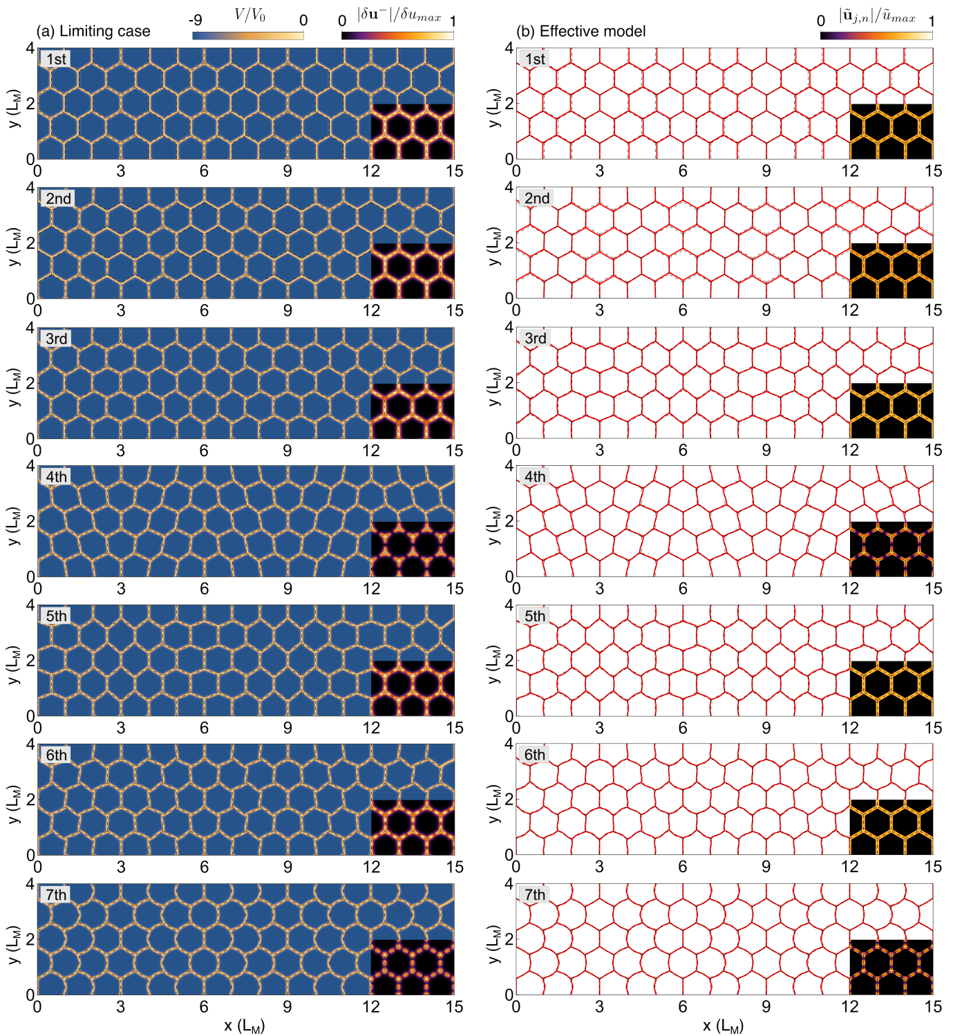
Figure 7. Phonon wave functions for the (a) limiting case and (b) effective model for the same modes and wave vectors as in Fig. 5. The corresponding total amplitude distributions for all wave vectors in MBZ is also shown as an inset.
