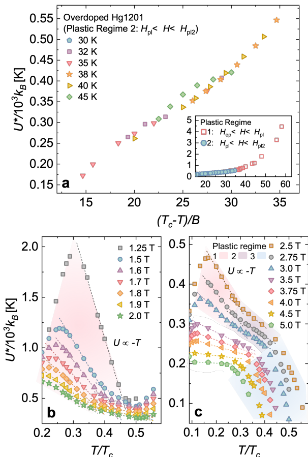
FIG. 7. (a) Energy scale U^* versus (T_c - T)/B for overdoped Hg1201 sample showing that data collapses onto a single curve such that U^* \sim 1/B in plastic regime 2. Inset shows collapse onto single curve for regimes 1 and 2. (a,b) U^* versus temperature, normalized to T_c , at (b) low fields and (c) higher fields. Plastic flow regimes 1, 2, and 3 identified by red, yellow, and blue shading, respectively. It is unclear whether the behavior in the unshaded region in (c) captures dynamics similar to regimes 1 or 2. Dashed lines are linear fits.
