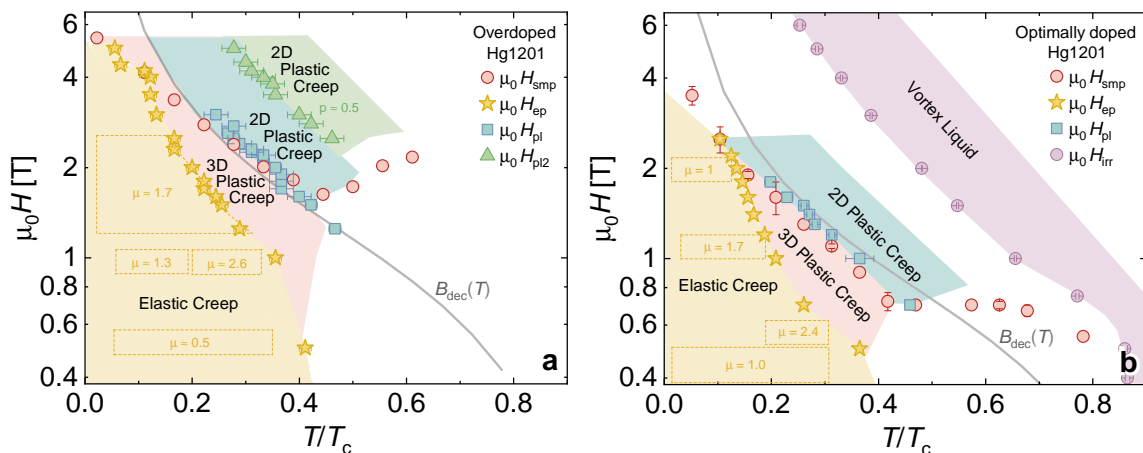
FIG. 8. Vortex phase diagram determined from creep measurements overlaid with position of second magnetization peak at H_{smp} for (a) overdoped and (b) optimally doped Hg1201 crystals. The gray curve is the prediction for the 3D-to-2D decoupling field based on Eq. 5. Overlap with B_{dec} suggests that the second magnetization peak originates from a 3D-to-2D dimensional crossover from 3D-to-2D plastic dynamics.
