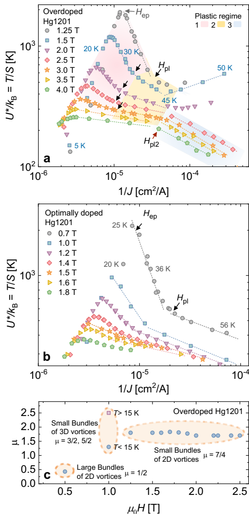
FIG. 5. (a) Energy scale U^* plotted against 1/J for the overdoped Hg1201 crystal measured in applied magnetic fields 1.25 T–4 T. Data was collected at 0.2 T intervals; for clarity, only select curves are displayed. Temperatures at which data was collected are noted for select data points: at fixed field, temperature increases with 1/J . Dashed lines are examples of linear fits used to extract glassy and plastic exponents, noted in Fig. 8 and the main text. Change from a positive to negative slope suggests a crossover from elastic to plastic vortex dynamics at H_{ep} . Data collected at fields below 3.2 T exhibit 2 kinks in the plastic flow regime at H_{pl} (lowest T kink, identified with black arrows) and H_{pl2} . Higher fields display only one kink, at H_{pl2} (example labeled with red arrow). Plastic flow regimes 1 ( H_{ep} < H < H_{pl} ), 2 ( H_{pl1} < H < H_{pl2} ), and 3 ( H > H_{pl2} ) identified by red, yellow, and blue shading, respectively. (b) U^* versus 1/J for the optimally doped Hg1201 crystal. (c) Field dependence of the glassy exponent in the overdoped sample. Labels indicate theoretical expectations that most closely match experimental values.
