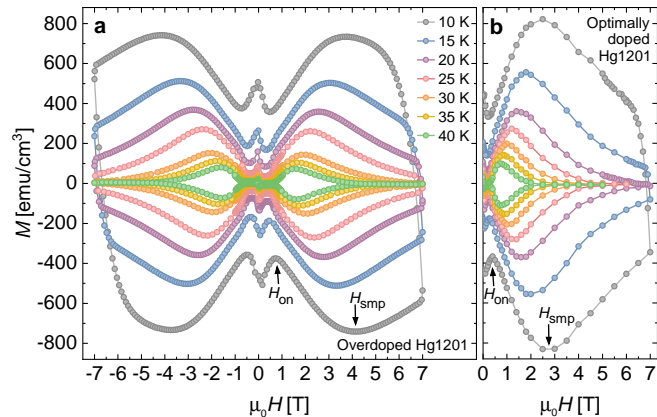
FIG. 3. Isothermal magnetic hysteresis loops M(H) at select temperatures for our (a) overdoped and (b) optimally doped Hg1201 single crystals. Each curve exhibits a second magnetization peak at H_{smp} and low-field dip at H_{on} .
