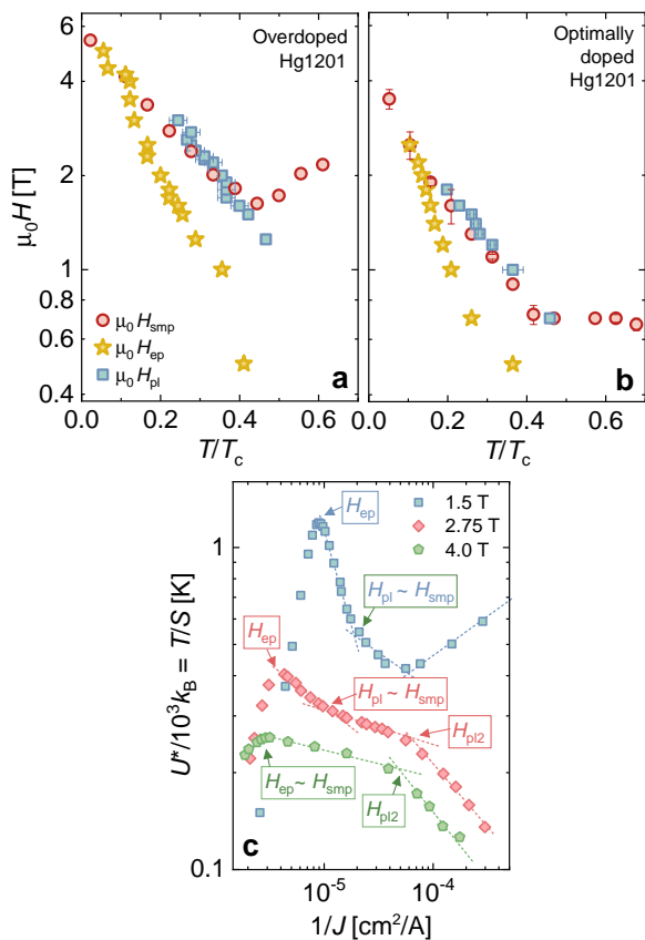
FIG. 6. Field - Temperature phase diagram for (a) overdoped and (b) optimally doped Hg1201 crystals showing that the second magnetization peak coincides with the elastic to plastic crossover only at high fields and with the kink in the plastic flow regime (at H_{pl} ) at lower fields. (c) U^* versus 1/J for overdoped Hg1201 crystal showing examples of 3 different types of behavior in plastic regime: low fields show two distinct negative slopes then an anomalous transition to a positive slope at low J ; intermediate fields display 3 distinct negative slopes; high fields exhibit 2 distinct negative slopes.
