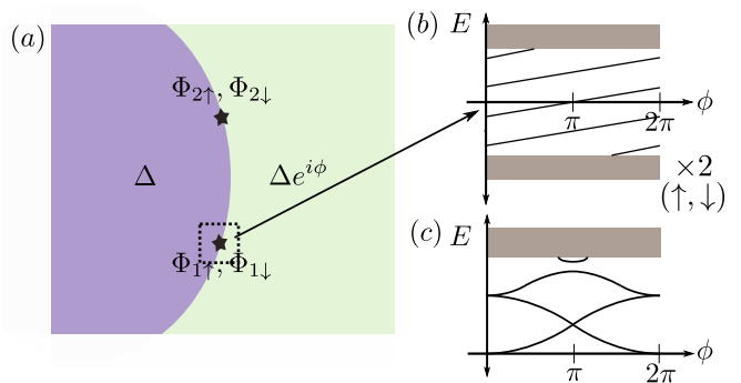
FIG. 3. Josephson junction for TBG-TSC. In (a), we apply a chemical potential via gate to shift the pairs of corner modes 1, 2 away from one another. At \phi = \pi , 4 total complex fermion corner modes (at the free fermion level) are pinned to zero energy, and breaking \mathcal{P} shifts the two pairs of two complex fermions in space. Varying the superconducting phase away from \pi will allow the corner modes to shift from zero energy, as depicted in (b), the single-particle spectrum (at finite chemical potential) for \Phi_{1\uparrow} . There is an identical copy of the spectrum for the opposite spin sector \Phi_{1\downarrow} , and doubled again for the other pair of in-gap modes \Phi_{2s} , though since that is separated in space we will not consider it. In (c), the multi-particle states involved in the ground state evolution are plotted. See SM for an in-depth discussion.
