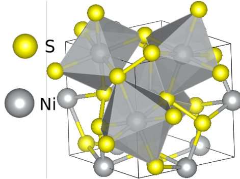
FIG. 1. The pyrite crystal structure. Grey and yellow atoms represent the transition metal (in this case Ni) and sulfur ions respectively. The Ni-S and S-S bonds have lengths of 2.39 \text{ \AA} and 2.07 \text{ \AA} respectively.
