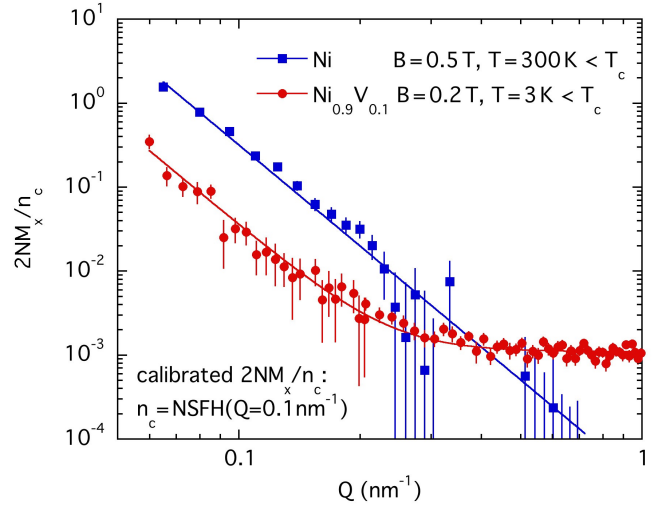
FIG. 16. Calibrated DIF response 2NM_x/n_c for Ni and \text{Ni}_{0.90}\text{V}_{0.10} vs. wave vector Q . In Ni only the long-range ordered domain term is present, the local defects appear in the V-alloy. The solid line is fit according to Eq. (8).
