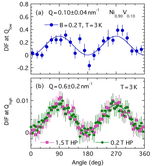
FIG. 10. Angle dependence of neutron response \text{DIF}(\theta) of \text{Ni}_{0.90}\text{V}_{0.10} for different Q -ranges at low T = 3 \text{ K} < T_c confirming magnetic response 2NM_x , solid lines follow Eq. (6). (a) Low Q -range covers (0.06 - 0.14) \text{ nm}^{-1} , (b) high Q -range includes (0.4 - 0.8) \text{ nm}^{-1} . HP denotes half polarized data, where \text{DIF} = \text{D} - \text{U} .
