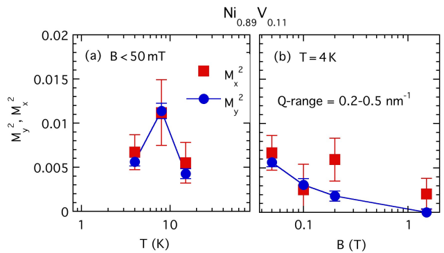
FIG. 8. Magnetic components M_y^2 and M_x^2 extracted from fit (Eq. (1)) of SF(\theta) data (shown in Fig. 6) of \text{Ni}_{0.89}\text{V}_{0.11} with T_c \approx 7 K at medium Q -range of (0.2-0.5) \text{nm}^{-1} . Panel (a) shows T -dependence of isotropic fluctuations in small fields ( B \leq 50 mT) and (b) shows B -dependence of short-range correlations at low T = 4 K, that are different for transverse and longitudinal components. Lines just connect data points.
