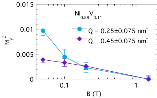
FIG. 9. Field dependence of magnetic component M_y^2 of \text{Ni}_{0.89}\text{V}_{0.11} at low T = 4 K. M_y^2 values estimated from SF(\theta) using Eq. (1) at two different Q -ranges as indicated. Lines just connect data.
