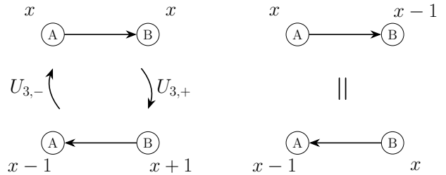
FIG. 7. Allowed game flips that correspond to 3-site dipole conserving operations. The game flips on the left correspond to U_{3,\pm} and the game flips on the right leave the scoring sequence unchanged and thus correspond to the identity operation.
