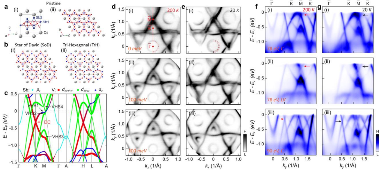
Fig. 1 | Crystal and electronic structures of \text{CsV}_3\text{Sb}_5 above and below T_{\text{CDW}} . a,b The crystal structure in the normal state (a), and CDW phase (b) with the candidate SoD structure (i) and TrH structure (ii). c DFT calculations for the orbital character resolved band structure. d,e CECs at different binding energies, measured at 200 K (d) and 20 K (e). f,g ARPES spectra obtained at 200 K (f) and at 20 K (g).
