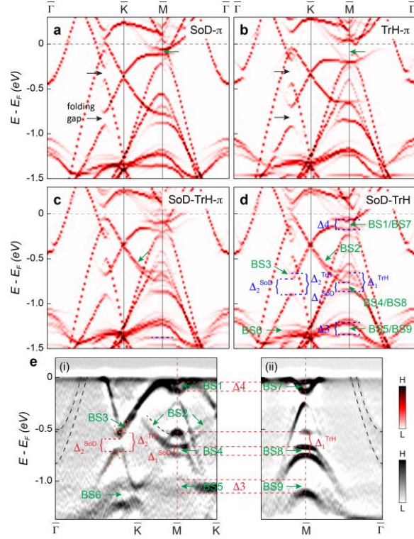
Fig. 4| Unfolded band structures in 2x2x2 CDW order from calculations. a-d The band structures of the following lattice configurations: SoD- \pi (a), TrH- \pi (b), SoD-TrH- \pi (c), and SoD-TrH (d). Blue dashed lines define the splitting gaps ( \Delta_1, \Delta_3, \Delta_4 ) and folding gaps ( \Delta_2 ). The superscripts SoD and TrH in the gaps ( \Delta_1, \Delta_2 ) represent the contributions of the two configurations, respectively. e ARPES spectra taken at 20 K along the \bar{\Gamma} - \bar{K} (i) and \bar{\Gamma} - \bar{M} (ii) directions.
