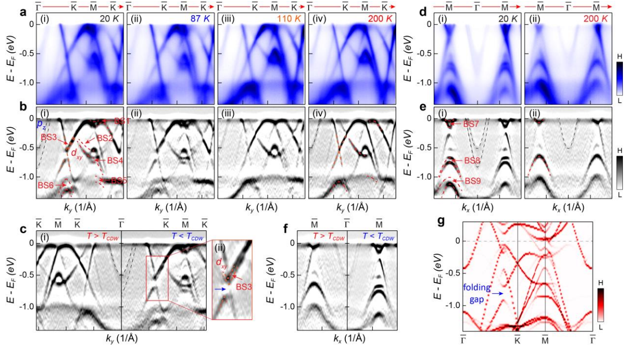
Fig. 3 | Double-band splitting features of kagome bands below T_{CDW} . a,b ARPES spectra (a) and their curvature plots (b) at different temperatures, taken along the \bar{\Gamma} - \bar{K} direction. c Comparison of the curvature plots taken at 200 K and 20 K. The orange box in (i) highlights the folding gap (ii). d-f Same as (a-c), but measured along the \bar{\Gamma} - \bar{M} direction. Red arrows indicate the double-band splittings in the CDW phase. g DFT calculations for the band structures of 2x2 TrH phase.
