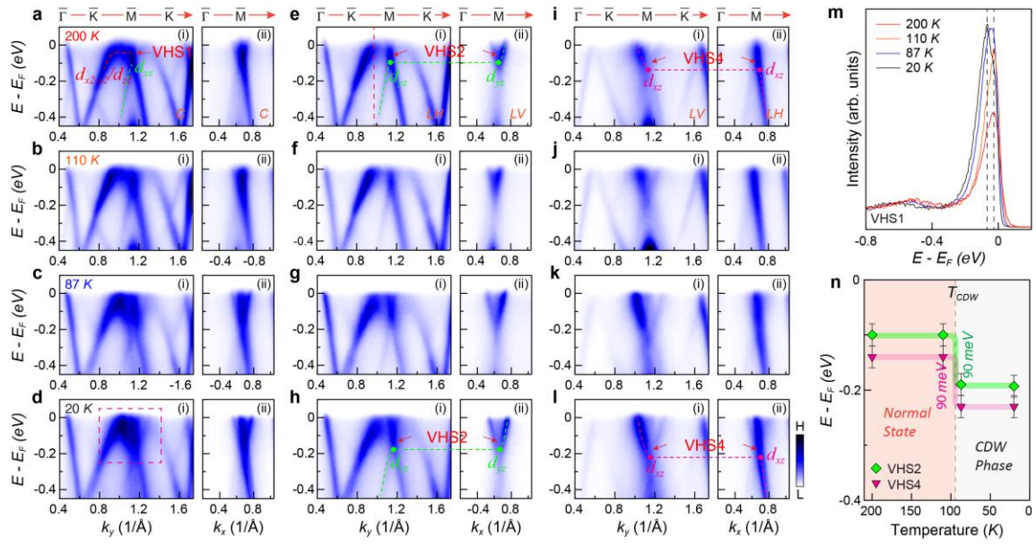
Fig. 2 | Temperature and polarization dependence of the electronic structure. a-d ARPES spectra taken along the \bar{\Gamma} - K [(i)] and \bar{\Gamma} - M [(ii)] directions, measured at 200 K (a), 110 K (b), 87 K (c), 20 K (d) with 78 eV C polarized light. e-h , i-l Same as (a-d), but obtained with LH [e-h(i), i-l(ii)] and LV [e-h(ii), i-l(i)] polarizations. Dashed curves are guide to the eye for the kagome bands around the M point. Red arrow indicates VHSs. m Temperature evolution of the EDCs taken around the flat feature of VHS1. The position of the EDCs is indicated by the red dashed line in [e(i)]. n Energy location of VHS2 and VHS4 as a function of temperature. The VHS positions are determined by the band bottom and top position at the M point.
