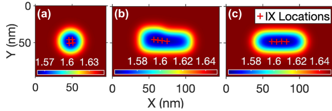
FIG. 4. Simulated locations for the 4-exciton state for a circular trap of diameter 35 nm (a), an oblong shaped hole whose dimensions most closely match that of the AFM topography (b), and an oval hole of 30 x 70 nm (c). Colorbar shows V_{IX}(x,y) , whose spatial profile is determined from the COMSOL simulation of the electric field underneath the etched graphene. The minimum and maximum V_{IX} are set based on the measured data from Figs. 2 and 3.
