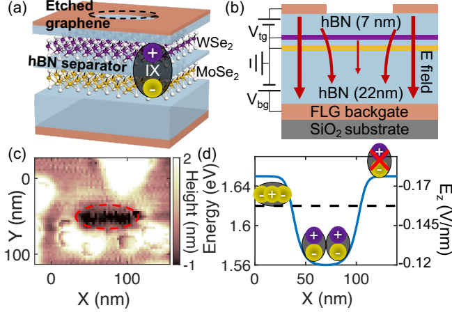
FIG. 1. Layout of the IX trapping structure. (a) Depiction of the \text{MoSe}_2 - \text{WSe}_2 heterostructure, with a thin hBN spacer layer, encapsulated in hBN with a patterned graphene top gate and FLG back gate. (b) Depiction of the spatially varying electric field through the heterostructure. (c) AFM topography of the etched graphene hole, with the etched area outlined by the dashed red line. (d) Diagram of the inter- and intra-layer exciton energy when the electric field is set such that the field away from the hole is -0.18 \text{ V/nm} . The IX energy shifts with electric field due to the permanent out-of-plane dipole moment, while the intralayer exciton energy is unchanged.
