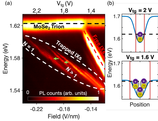
FIG. 2. (a) PL from a single IX QD as a function of electric field, with excitation power 125 nW. The trapped IX PL shows discrete narrow emission lines, and energy shifts with electric field shown by green arrows. The electric field axis refers to electric field strength away from the etched graphene. (b) Exciton energy near the etched graphene for varying applied voltage. Blue line indicates IX energy, black dashed line indicates MoSe 2 trion energy. Red lines mark the intersection, showing that with increasing applied voltage, there is less area where excitons will fall to the trapped IX state.
