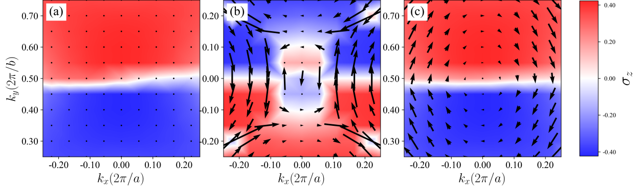
FIG. 3. Spin texture of outer branch of the lowest conduction bands for GMG around \Gamma (panels a and b) and Y(0.0, 0.5, 0.0) (panels c) points. Panel (a) shows the spin texture at zero external electric field. Panel (b) and (c) display the spin texture at an electric field of 0.1 \text{ eV/\AA} . The black arrows represent in-plane spin component, while blue and red color represent the out-of-plane spin component.
