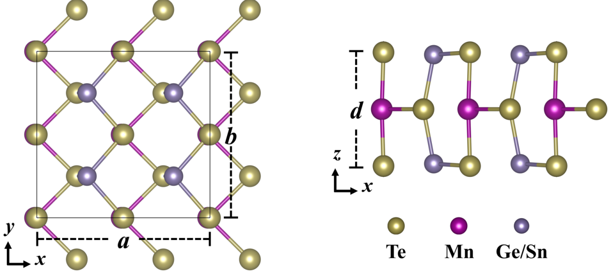
FIG. 1. Structure of XMN. The left and right panels show the top and side view, respectively. Note that there are four Mn ions in the supercell, which is represented by a rectangle.
