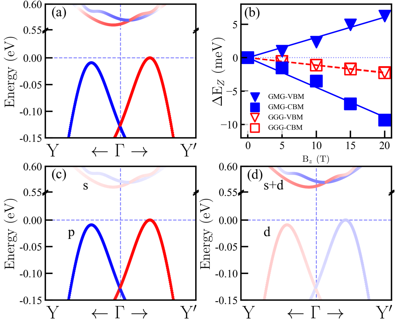
FIG. 4. (a) The band structure of GMG at Y- \Gamma -Y' under an out-of-plane magnetic field of 20T, and (b) Zeeman-splitting energy as a function of out-of-plane magnetic field. (c) Te and (d) Mn projected band structure of panel (a). The color depth indicates the quantity of the projected contribution.
