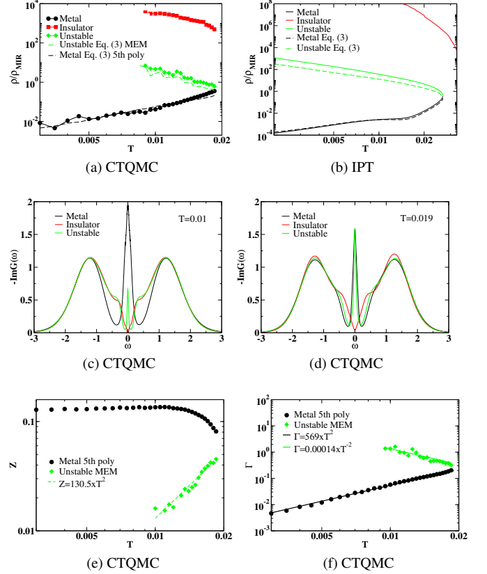
FIG. 3. The resistivity for the metallic (black circles), insulating (red squares), and unstable (green diamonds) solutions along the constant U trajectory in logarithmic \rho scale for (a) CTQMC and (b) IPT. The Sommerfeld approximations to the resistivities [Eq. (3)] are shown in the corresponding dashed and dotted lines with different analytic continuation methods (MEM and polynomial fitting for CTQMC and Padé approximant for IPT). The density of states at low temperatures (c) T = 0.01 and (d) T = 0.019 near the spinodal line U_{c2} computed from the CTQMC impurity solver and MEM analytic continuation. (e) The quasiparticle weight, Z , for the metallic and the unstable solutions. (f) The scattering rate \Gamma for the metallic and the unstable solutions.
