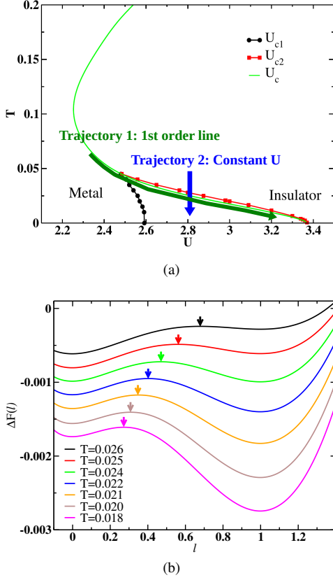
FIG. 1. (a) DMFT phase diagram for the half-filled Hubbard model and the trajectories studied (see text). (b) The evolution of the free energy functional [30] as T varies for the fixed- U trajectory ( U = 2.83 ). Here l = 0 and l = 1 correspond to the insulating and metallic solutions, respectively. The arrows mark the position of the unstable solutions.
