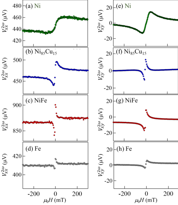
FIG. 2. Magnetic field dependence of V_{xx}^{2\omega} and V_{xy}^{2\omega} for (a, e) Ni/Pt, (b, f) \text{Ni}_{85}\text{Cu}_{15} /Pt, (c, g) \text{Ni}_{81}\text{Fe}_{19} /Pt, and (d, h) Fe/Pt bilayers. The current density j_c was fixed at 0.87 \times 10^{11} \text{ A/m}^2 .
