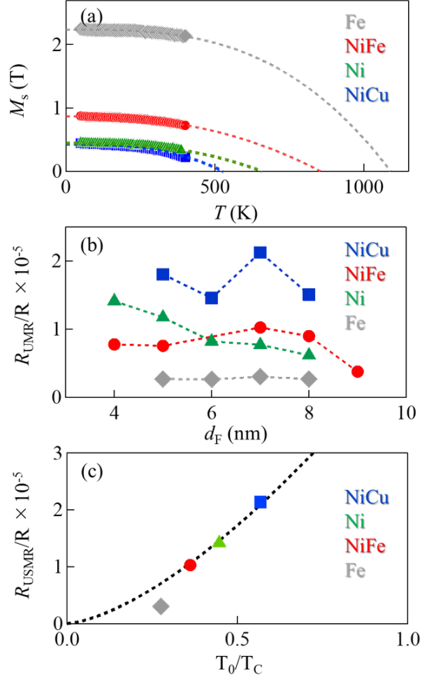
FIG. 5. (a) Temperature dependence of the magnetization for each FM film. (b) FM thickness dependence of R_{\text{USMR}}/R (c) Curie temperature dependence of R_{\text{USMR}}/R for the FMs/Pt bilayer. Dashed line is the fitting curve using R_{\text{USMR}}/R = A(T_0/T_C)^\alpha . Here, A and \alpha is the proportionality constant and exponent, respectively.
