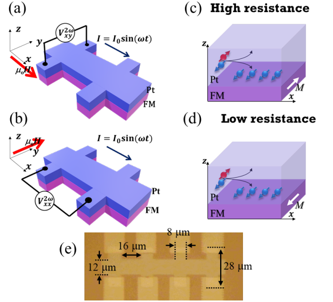
FIG. 1. Schematic experimental setup for measuring the second harmonic of (a) transverse and (b) longitudinal voltages, i.e. V_{xy}^{2\omega} and V_{xx}^{2\omega} , with applying external magnetic field along x - and y -axes, respectively. (c) High- and (d) low-resistance states of the FM/Pt bilayer film owing to the USMR effect. (e) Optical microscopic image for our device.
