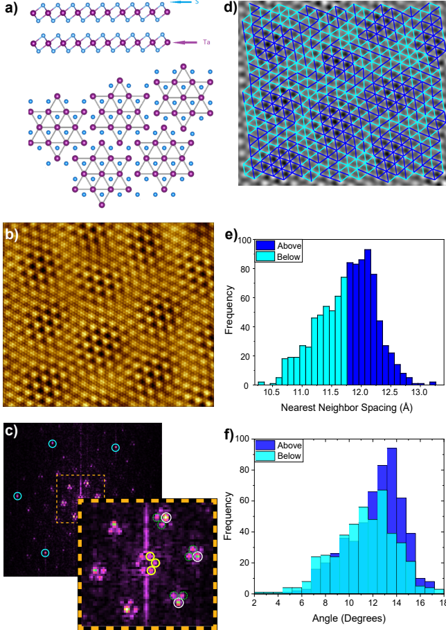
FIG. 1. a) Top: Layered crystal structure for 1T-TaS 2 . Bottom: Top view showing Ta-formed David stars. Surface S ions, directly imaged by STM, are superimposed for reference. Crystal structure created using Vesta.[27] b) 230 Å x 200 Å STM topography ( I = 450 pA and V_{Bias} = 150 mV). Image was Fourier filtered to include signals identified in (c). Zoom of single domain in supplemental material.[28] c) Fourier transform of 230 Å x 200 Å topographic image at left. Atomic signals are circled in blue. Large orange dotted square is zoom of central FFT region. Within this central region are low wavevector peaks (yellow) and average CDW peaks (white) around which there are satellite peaks (dotted green). d) Connections between NN CDW maxima superimposed on Fourier filtered topographic image (now grayscale). Filtered image shows only locations of CDW maxima. Average NN distance is 11.76 Å. Blue (cyan) connections show NN separations above (below) 11.76 Å threshold. e) Histogram of NN distances with 0.1 Å bin size, reflecting image resolution. f) Angles of NN connectors relative to atomic lattice. Blue (cyan) show angular distributions for connectors above (below) 11.76 Å threshold.
