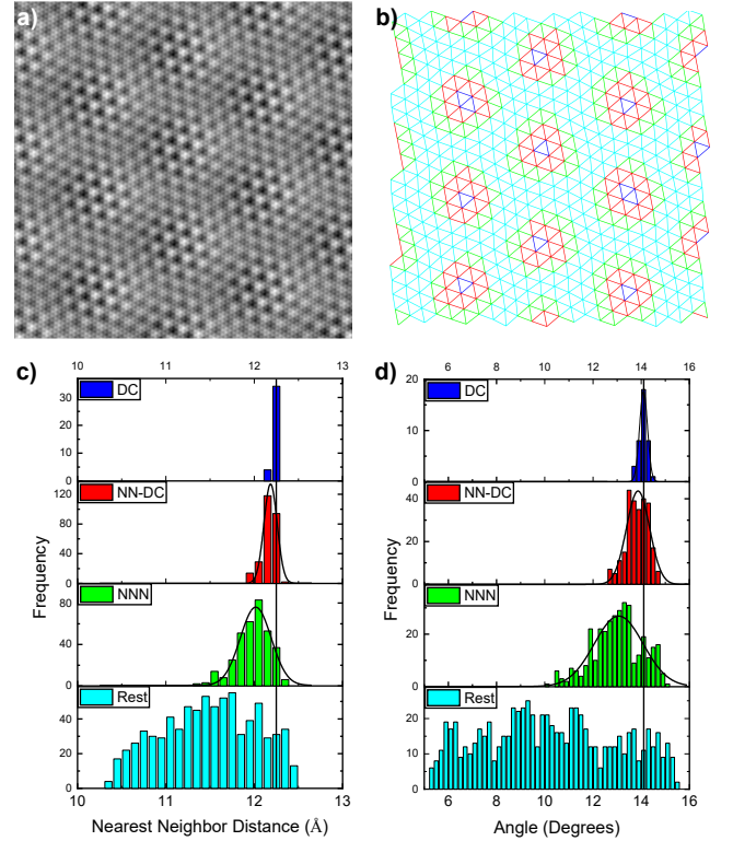
FIG. 3. a) 253 \text{ \AA} \times 253 \text{ \AA} computer-simulated STM topography. Average intensity and wavevectors for atomic, CDW, satellite, and low-wavevector peaks from Figure 1c were used to create image (supplemental materials [33]). b) From intensity thresholding: Domain center (blue). NN-DC (red) nearest neighbor CDW connectors towards domain center (excludes blue connectors). NNN (green) next nearest neighbor connectors towards domain center (excludes blue and red). Rest (cyan) remaining connectors (excludes blue, red, green). c) Histograms of NN distances for each connector grouping. Statistics: 11.48 \pm 0.53 \text{ \AA} (cyan) to 11.98 \pm 0.19 \text{ \AA} (green) to 12.16 \pm 0.08 \text{ \AA} (red) to 12.23 \pm 0.03 \text{ \AA} (blue) d) Histograms of CDW angles relative to atomic lattice for each connector grouping. Statistics: 10.2^\circ \pm 2.7^\circ (cyan) to 13.0^\circ \pm 1.0^\circ (green) to 13.8^\circ \pm 0.5^\circ (red) to 14.1^\circ \pm 0.2^\circ (blue). Gaussian fits and vertical line at DC peak are superimposed in c) and d) to illustrate evolution of peak location and width.
