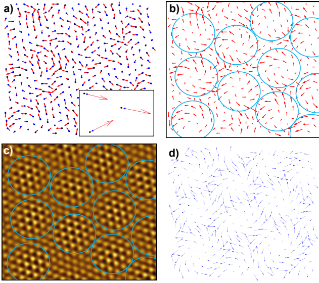
FIG. 4. a) Arrows point from CDW_{ave} maxima to nearest CDW_{ltc} maxima. Arrow length is proportional to displacement. Inset shows zoom and illustrates arrows pointing from CDW_{ave} maximum (black) to CDW_{ltc} maximum (blue). b) Blue circles are superimposed on arrows from a) as a guide to the eye to show the vortex-like chiral displacement patterns. c) The same blue circles are superimposed on CDW_{ltc} topography and match domain locations. d) Arrows are drawn from the CDW_{ave} maximum location to the nearest imaged sulfur ion. An identical, though translated, pattern is produced if arrows are drawn from CDW_{ave} maxima locations to the nearest Ta ions (supplemental material [34]). We chose the sulfur ion for this figure since we image those ions directly and obtain the same information. Note, while the Lawler-Fujita algorithm has proven useful in extracting picometer-scale drift and lattice strain fields,[35, 36] it is not suitable for use in extracting the local displacement fields shown in this figure (supplemental material [37]).
