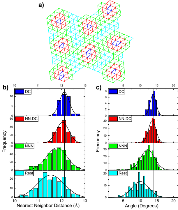
FIG. 2. a) Domain center (blue) found using local intensity thresholding. NN-DC (red) nearest neighbor CDW connectors towards domain center (excludes blue connectors). NNN (green) next nearest neighbor connectors towards domain center (excludes blue and red). Rest (cyan) remaining connectors (excludes blue, red, green). Domains with centers near the edge of the topography are ignored. b) Histograms of NN distances for each connector grouping with 0.2 \text{ \AA} bin size. c) Histograms of CDW angles relative to atomic lattice for each connector grouping. Gaussian fits and vertical line at DC peak are superimposed in b) and c) to illustrate evolution of peak location and width.
