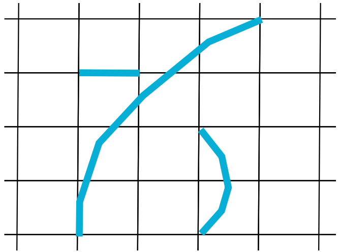
FIG. 1: A cartoon figure illustrating the structure of resonances in the critically localized phase. Spins live on every vertex of the lattice shown above. Thick blue lines connect spins that are in resonance. Resonances exist on all lengthscales, but do not percolate.
